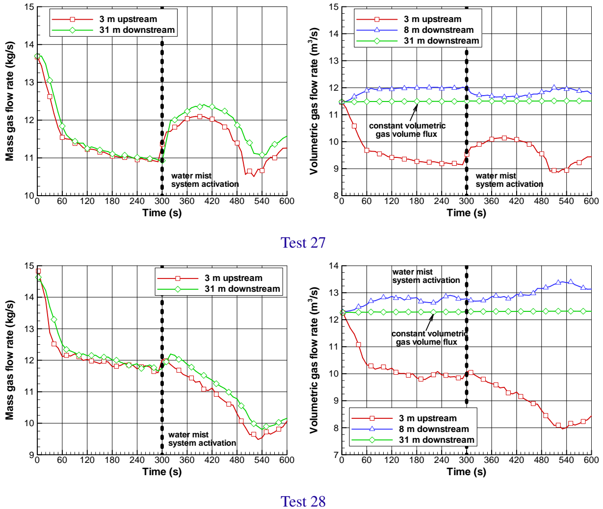
Fig. III.32 — Gas flow rates versus time in mass (left) and in volume (right) simulated at several distances from the fire
