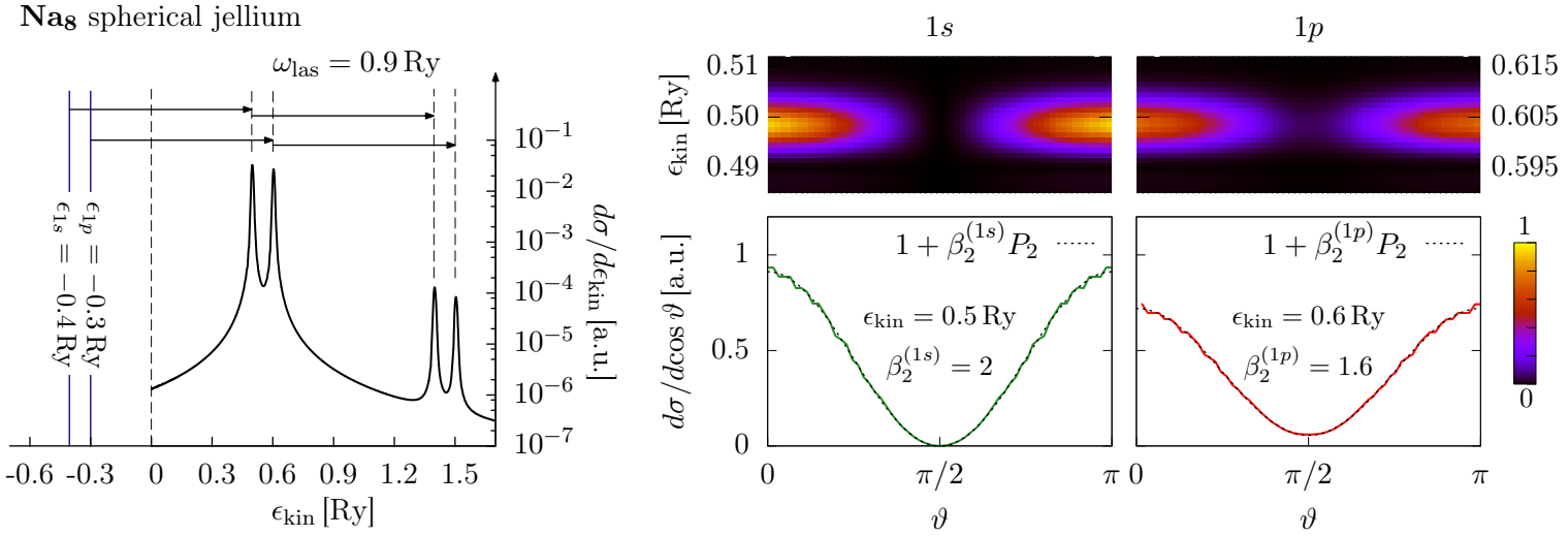
Figure 5.1: Spectrum and angular distributions of photoelectrons in Na 8 spherical jellium ( r_s = 3.65 a_0 , \sigma_{\text{jel}} = 1 a_0 , \epsilon_{1s} = -0.405 Ry, \epsilon_{1p} = -0.300 Ry) after excitation with a 60 fs linearly polarized laser pulse of I = 6.9 \times 10^{13} W/cm 2 and \omega_{\text{las}} = 0.9 Ry. The total ionization is N_{\text{esc}} = 0.003 electrons. The angle \vartheta is measured with respect to the laser polarization axis. The s.e. wavefunctions have been stored at a very large number of measuring points, M = 137 , all along one longitude due to the \varphi -symmetry. PES and PAD are so determined by Fourier transformation of the same observable.
