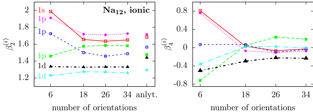
Figure 5.17: Single-electron anisotropies \beta_2^{(i)} (left) and \beta_4^{(i)} (right) for Na 12 excited by strong laser pulse in the non-linear regime. Results are drawn as a function of the number of averaging orientations.
