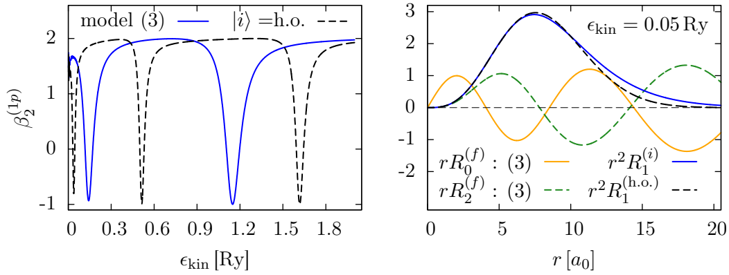
Figure 6.7: Left panel: Anisotropy of the 1p shell in \text{Na}_8 spherical jellium within model (3) (blue line). Replacing the initial self-consistent state by the harmonic fit yields the black, dashed line. Right panel: Continuum waves rR_0^{(f)} and rR_2^{(f)} within model (3) at energy \epsilon_{\text{kin}} = 0.05 \text{ Ry} , initial self-consistent wavefunction r^2R_1^{(i)} , and harmonic fit function r^2R_1^{(\text{h.o.})} .
