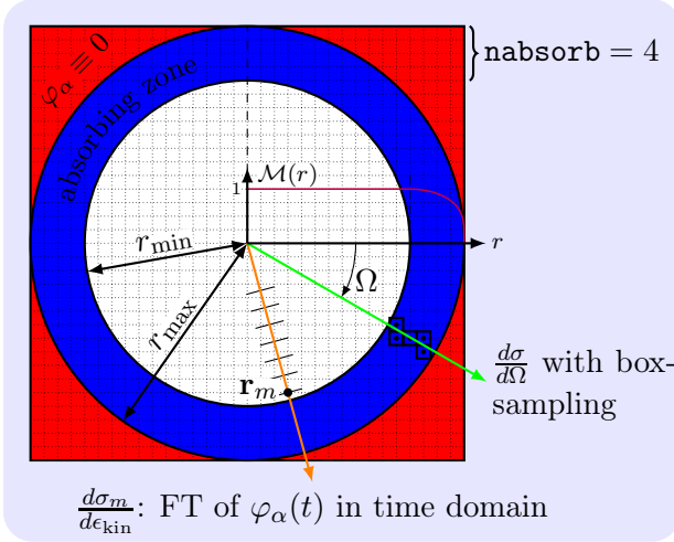
Figure 3.2: Illustration of the spherical absorbing boundaries. The parameter \mathbf{nabsorb} = (r_{\max} - r_{\min})/\Delta x gives the width of the absorbing layer. The cross-section d\sigma/d\Omega can be calculated through representation of each absorption point with a weight function \mathcal{W} (in the figure box-like). The measuring points \mathbf{r}_m of the PES are just before the boundary starts.
