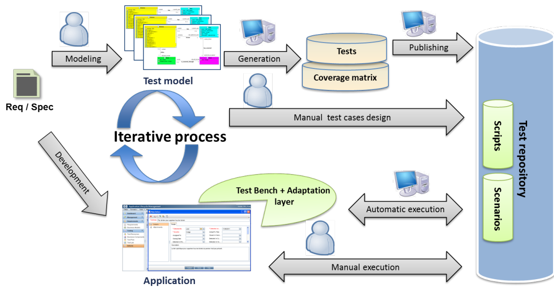
FIGURE 1.1 – Model-Based Testing
