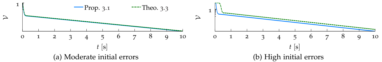
Figure 3.6: Exponential convergence of the errors – logarithmic \gamma -scale.
