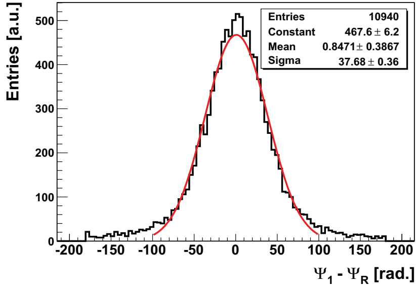
Figure 7.14: Distribution of the difference between the reconstructed event plane ( \Psi_1 ) and the true reaction plane ( \Psi_R ) in semi-peripheral Au + Au events ( 6 < b < 8 fm) at a beam energy of 25 GeV/nucleon. The red line is a Gaussian fit to the distribution.
