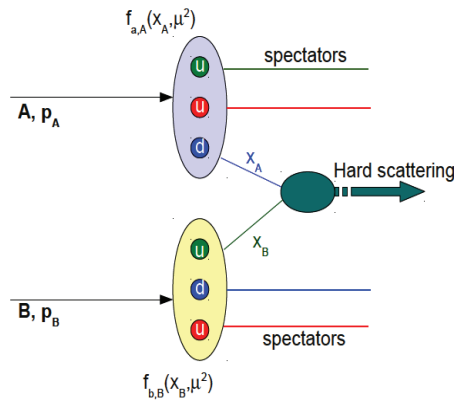
Figure 1.8: Illustration of a pp collision. The two protons, (A,B), are each made out of three partons (uud). Only a pair of the constituent partons are involved in the hard scattering, and they carry a fraction of the momentum of the incident proton (A,B) equal to x_a and x_b respectively.
