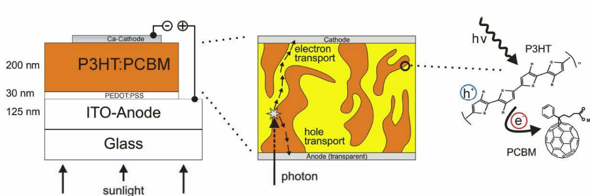
Figure 6, General structure and basic principle of the BHJ solar cells. Electron donor poly(3-hexylthiophene) (P3HT) and acceptor (PCBM) are blended together to maximize the interface where the exciton dissociation into electrons and holes takes place. For an efficient photocurrent, each material must provide a continuous path for electron and hole transport to the respective contact 15 .
