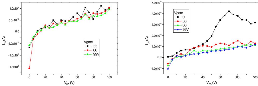
Figure 2 , I-V characteristics of 18 for (left) 20 \mu m and (right) 2.5 \mu m channel lengths at different gate voltages after annealing.
