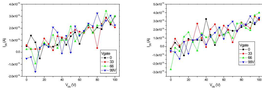
Figure 3 , I-V characteristics of 16 for (left) 20µm and (right) 2.5µm channel lengths at different gate voltages before annealing.
