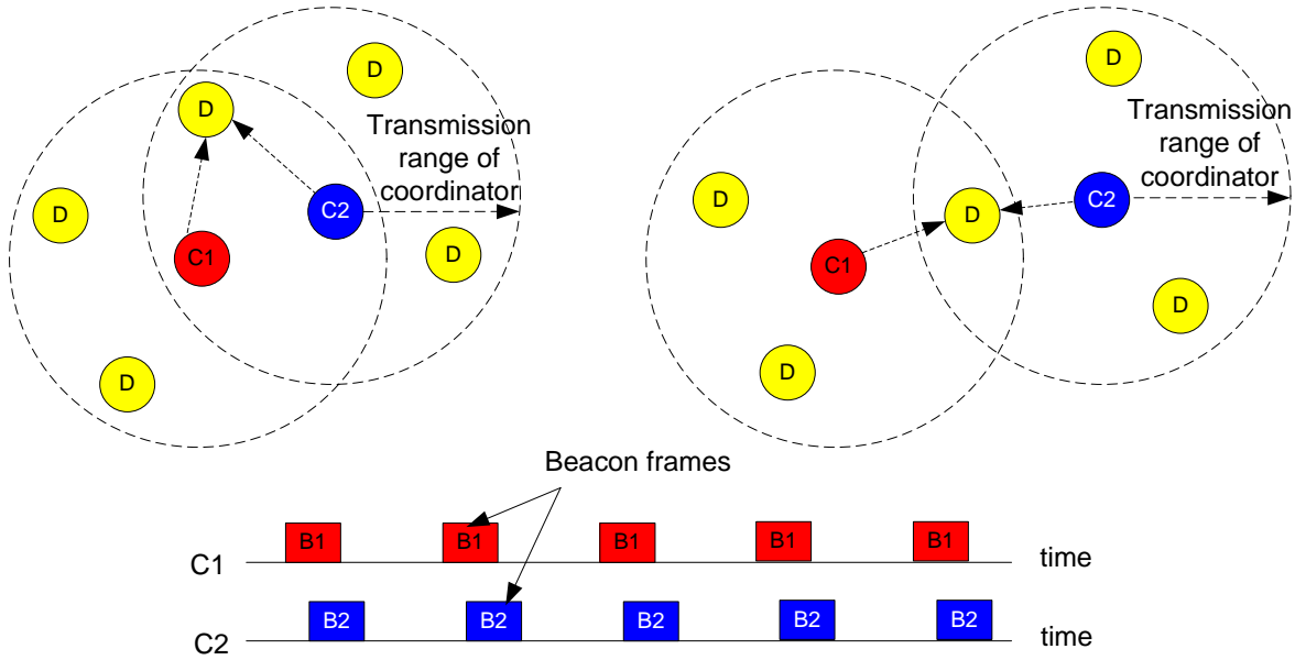
Figure 1.15 Beacon collision
