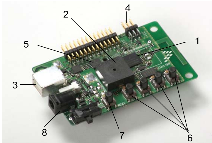
Figure 4.3 1321x-SRB node
