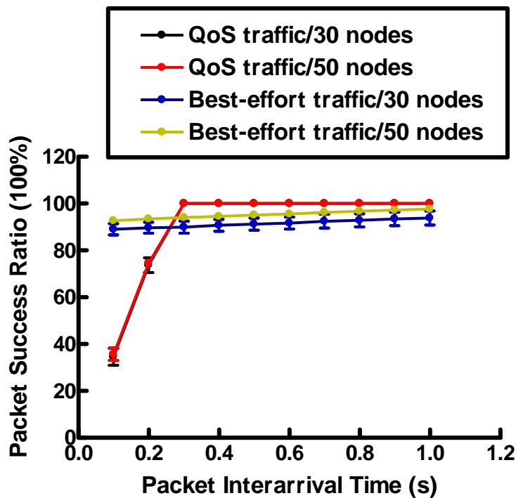
Figure 3.24 Packet success ratio for different scale
