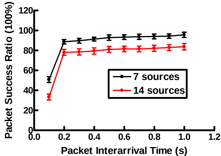
Figure 3.16 CSMA/CA packet success ratio with different sources
