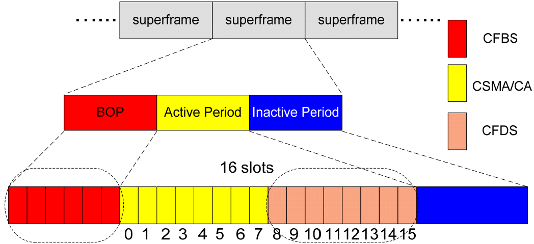
Figure 2.2 ADCF superframe structure
