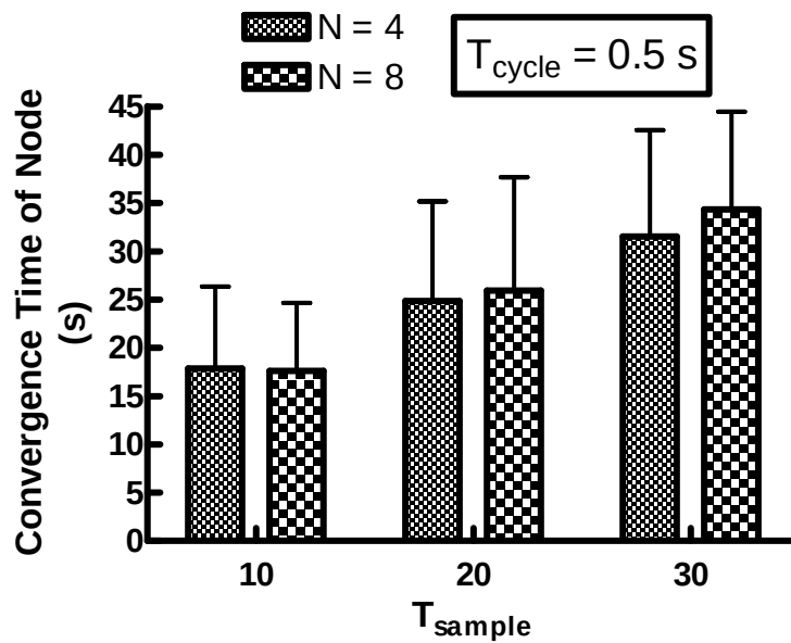
Figure 4.14 Convergence time vs. T_{sample}
