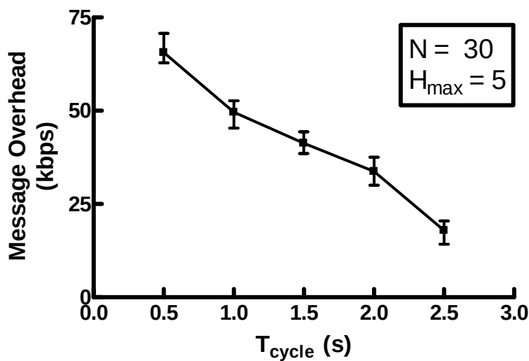
Figure 3.10 Message overhead vs. T_{\text{cycle}}
