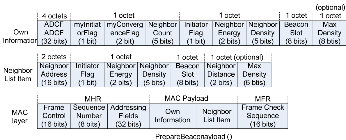
Figure 4.8 Beacon frame format for prototyping
