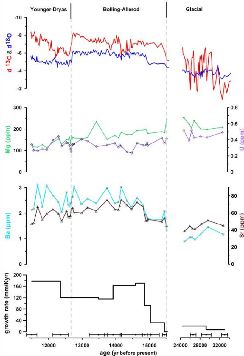
Fig. 2. Chau-stm6 stable isotopes, Mg, U, Ba and Sr concentrations versus age. Concentrations are presented in Supplementary materials and U–Th ages with 2\sigma errors are derived from (Genty et al., 2006). The 13.5 ka Mg peak was not replicated and is not considered in the discussion, while the 15.5 Mg peak is considered meaningful, given that it is similar to glacial levels, and the other elements and stable isotopes peaking or troughing at the same time. Chau-stm6 stable isotopes, Mg, U, Ba and Sr concentrations versus age. Concentrations are presented in Supplementary materials and U–Th ages with 2\sigma errors are derived from (Genty et al., 2006). The 13.5 ka Mg peak was not replicated and is not considered in the discussion, while the 15.5 Mg peak is considered meaningful, given that it is similar to glacial levels, and the other elements and stable isotopes peaking or troughing at the same time.
