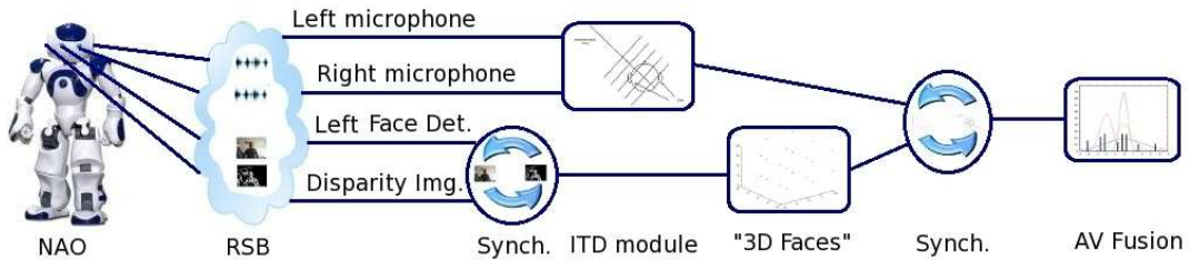
Figure 7.4: Modular structure of the audio-visual fusion algorithm. Data coming from left and right microphones is processed and used to compute the ITDs. Left face detection and the disparity map are synchronized and used to extract 3D position of each detected face by the 3D Faces module. Finally, to proceed to the fusion, these faces are synchronized with previously computed ITDs. A last module for visualization is explained later, see Fig. 7.5.
