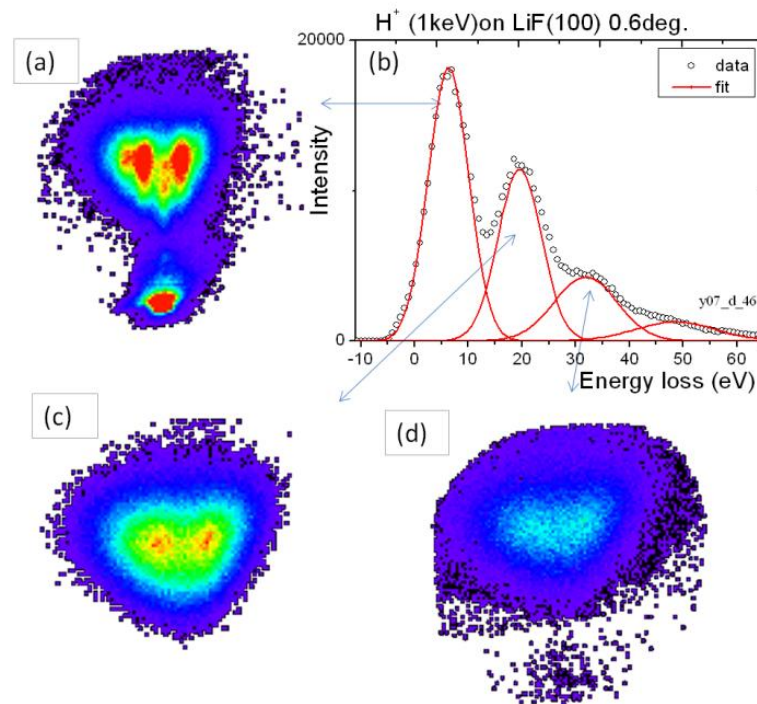
Figure 6.24 Angular distributions recorded with position sensitive detector and energy loss spectrum via TOF for scattering of 1keV H^+ ions from LiF(001) under \theta_{in}=0.6deg. along LiF<100>orientation. (a) 2D scattering intensity of outgoing H^+ associated to only neutralization on LiF surface; (b) energy loss spectrum, (c) intensity coincident with energy loss around 20eV; (d) intensity coincident with energy loss around 35eV. ( a=0.13 )
