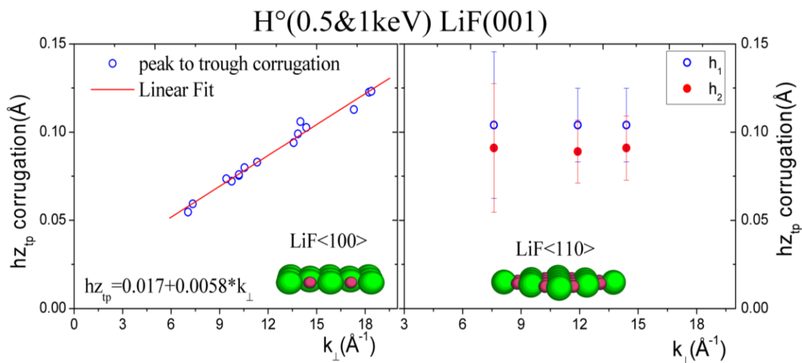
Figure 6.20 Corrugation from trough to peak increases linearly with impact vector normal to surface along \text{LiF} surface \langle 100 \rangle , but slightly decreases along \langle 110 \rangle direction, note that their scales are not the same.
