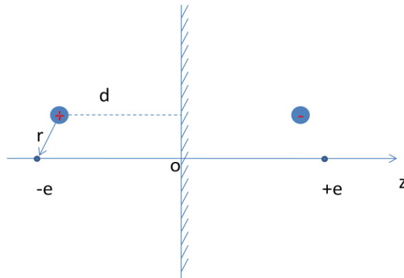
Figure 3.22 Ion and its image charge located symmetrically beside surface plane.
