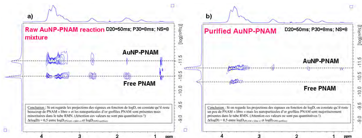
Figure III. 18: ^1H -DOSY NMR charts of: a) Raw AuNP-PNAM reaction mixture in D_2O ; b) Purified AuNP-PNAM in D_2O .
