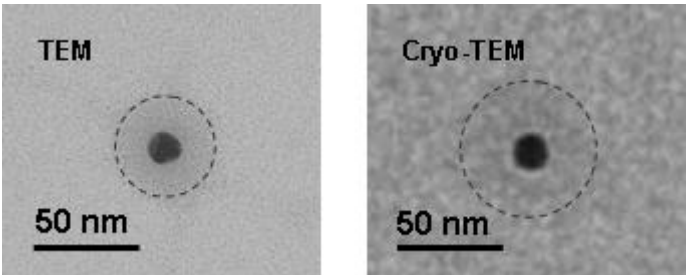
Figure III. 39 : Comparison between (left) classical TEM with RuO 4 staining; (right) cryo-TEM (no staining) on one grafted nanoparticles of AuNP-LY32KDa(B) sample.
