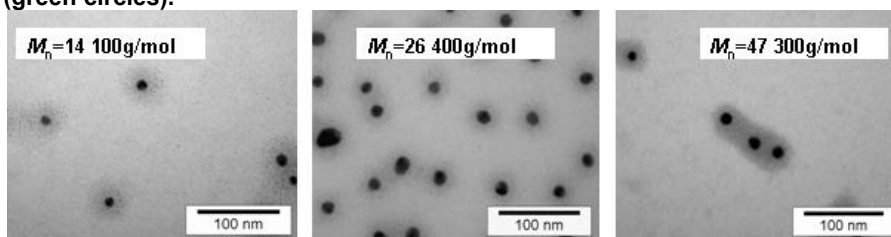
Figure III. 30 : TEM images of AuNP-PNAM obtained by ligand exchange respectively with M_n = 14\ 100 / 26\ 400 / 47\ 300\ \text{g.mol}^{-1} (staining with \text{RuO}_4 ).
