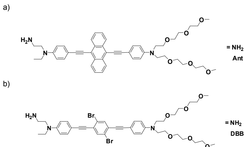
Figure II. 21: Chemical structure of a) Ant and b) DBB chromophores.
