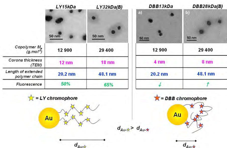
Figure IV. 40: Possible conformations of grafted TP conjugates vs. LY conjugate onto AuNP.
