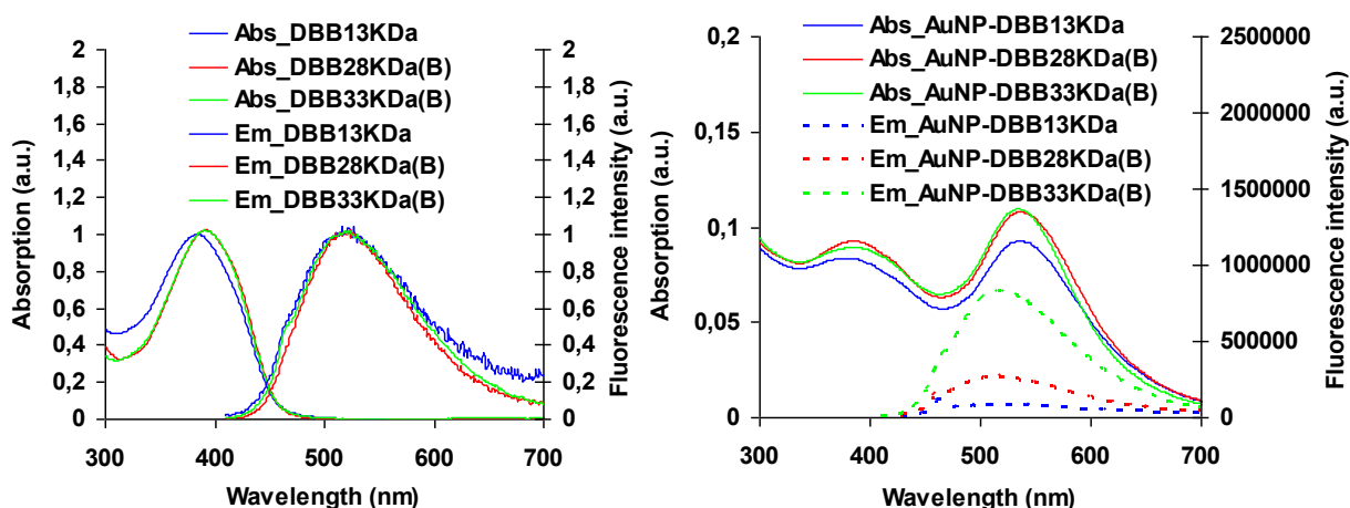
Figure IV. 37: Absorption/Emission spectra of DBB conjugates before (left) and after (right) grafting onto AuNP ( \lambda_{ex}=400\text{nm} ).
