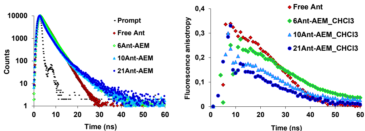
Figure IV. 21: Fluorescence lifetime (left graph) and anisotropy (right graph) of Ant-polymer conjugates compared to free Ant chromophore in \text{CHCl}_3 ( \lambda_{\text{ex}}=469\text{nm} ; \lambda_{\text{em}}=560\text{nm} ).
