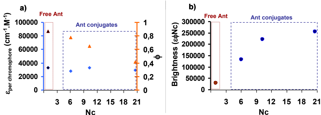
Figure IV. 15: Influence of the number of Ant chromophores per chain ( N_c ) on: a) molar extinction coefficient ( \epsilon ) and fluorescence quantum yield ( \phi ); b) and on brightness of Ant-polymer conjugates in \text{CHCl}_3 . Comparison with free Ant chromophore.
