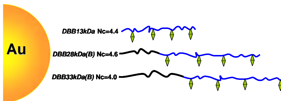
Figure IV. 36: DBB conjugates with different polymer lengths and different DBB density/chain used for grafting onto 20 nm AuNP: DBB13KDa – random copolymer; DBB28KDa(B) –block copolymer with 8 000 \text{g.mol}^{-1} spacer; DBB33KDa(B) – block copolymer with 12 000 \text{g.mol}^{-1} spacer.
