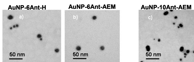
Figure III. 36 : TEM images of ~20 nm AuNP grafted with Ant-conjugates: a) 6Ant-H; b) 6Ant-AEM; c) 10Ant-AEM casted from CHCl 3 solution (staining with RuO 4 ).
