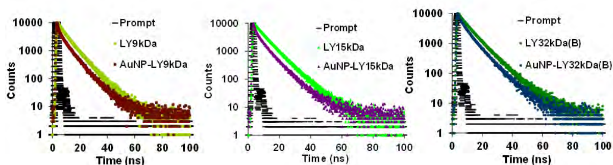
Figure IV. 34: Fluorescence decays of grafted AuNP vs. free LY conjugates: (left) AuNP-LY9KDa, (middle) AuNP-LY15KDa, (right) AuNP-LY32KDa(B), ( \lambda_{\text{ex}}=440\text{nm} , \lambda_{\text{em}}=530\text{nm} , ).
