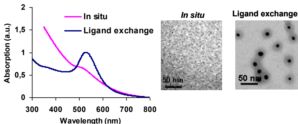
Figure III. 31 : (left) Comparative UV-Vis spectra of 2 nm AuNP-PNAM by in situ approach vs. ~20 nm AuNP-PNAM grafted by ligand exchange. (right) TEM images corresponding to in situ vs. ligand exchange grafted AuNP (black dots or spheres are AuNP cores).
