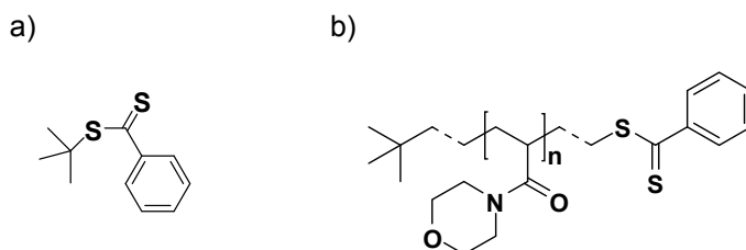
Figure II. 4: a) Molecular structure of t BDB; b) Structure of PNAM synthesized by RAFT using t BDB as CTA.
