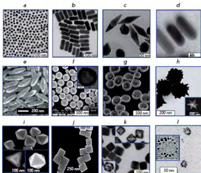
Figure I. 10: Various types of AuNP: a) 16nm spherical AuNP; b) Au nanorods; c) Au bipyramids; d) Au nanorods with silver coating; e) Nanorice – \text{Fe}_2\text{O}_3 nanorods covered by a Au nanoshell; f) Au nanoshell onto silica core; g) nanobowls, with Au seeds on the bottom; h) spiky nanoshell with \text{SiO}_2/\text{Au} shells (inset: star NP); i) polyhedral AuNP; j) Au nanocubes; k) Au-Ag nanocages; l) nanonecklaces. 60
