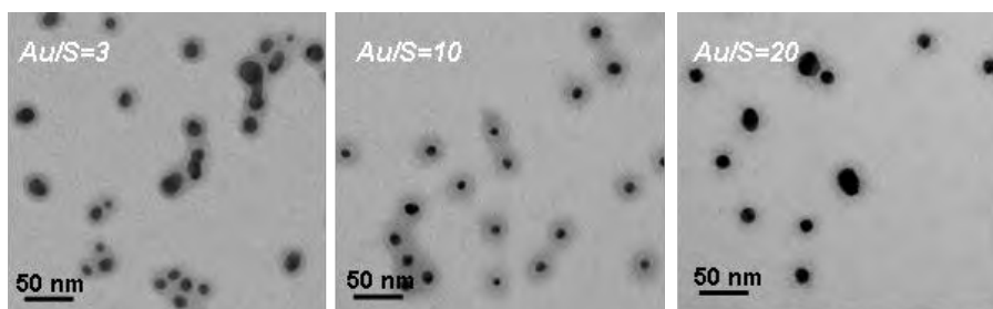
Figure III. 27 : TEM images of PNAM ( M_n=14\,000 g/mol) grafted by ligand exchange onto AuNP using Au/S ratio = 3, 10, or 20 respectively (staining with \text{RuO}_4 ).
