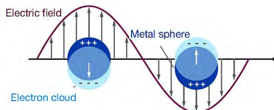
Figure I. 8: Schematic diagram of localized SPR. 54
