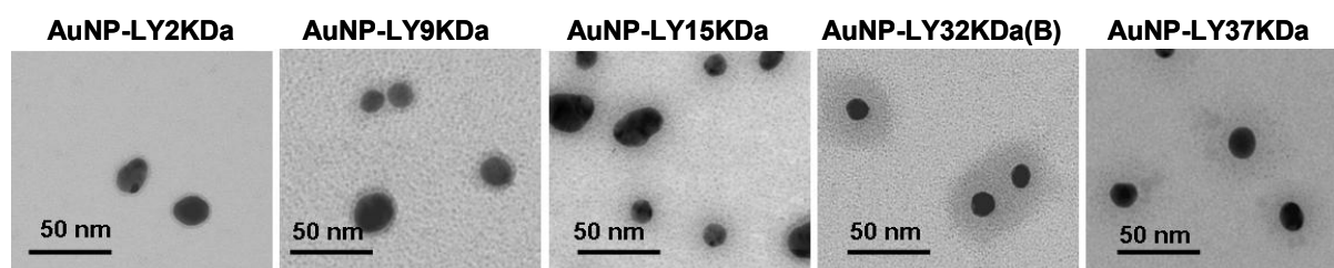
Figure III. 35 : TEM images of ~20 nm AuNP grafted with LY-conjugates having different lengths (staining with RuO 4 ).
