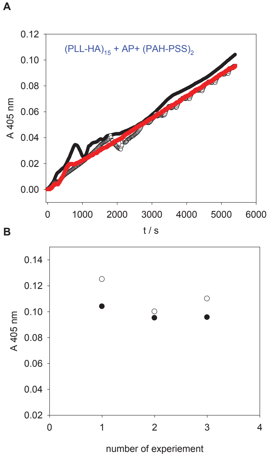
Figure 37. A. Evolution of the absorbance at 405 nm of a (\text{PLL-HA})_{15} film loaded with the enzymes (AP) during 2h, with a (\text{PAH-PSS})_2 capping layer and put successively in a 3 mM PNP containing Tris-NaCl buffer, for the first (●), the second (○) and the third measurement (■). After each experiment the film was immersed in Tris-NaCl buffer to wash away PNP and the corresponding hydrolysis product.
