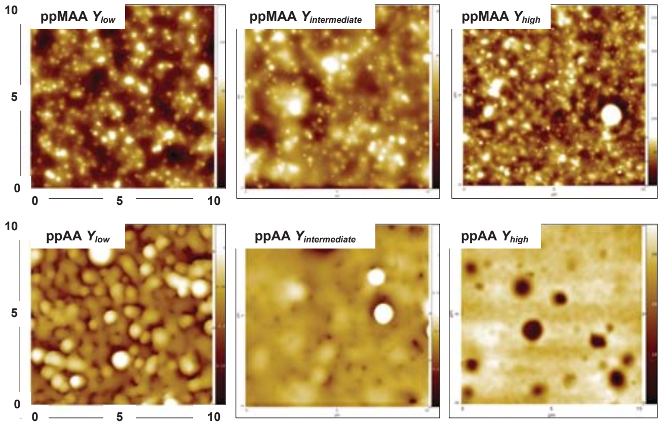
Figure 20. Typical AFM topography images (10µm x 10µm) obtained from coatings made from AA and MAA under different value of Y and after 80 passes.
