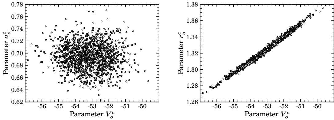
Figure 4.30: The results of Monte Carlo fitting for ^{208}\text{Pb} projected on the ( a_0^c vs. V_0^c ) plane (left) and ( r_0^c vs. V_0^c ) plane (right).
