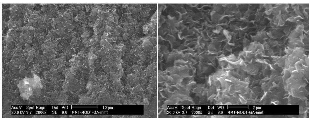
Figure 4.49 : SEM pictures of the clay-rich fraction of PCL/montmorillonite nanohybrid obtained from the polymerization catalyzed by MMTMODL G and showing the PCL chains grafting on clay surface at 2000x magnification (left) and 8000x magnification (right).
