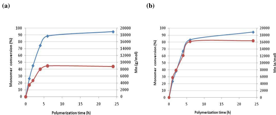
Figure 4.9 : Time-evolution curves of \epsilon -CL conversion ( \blacklozenge ) and molecular weight ( M_n ) of obtained PCL ( \bullet ), as determined by ^1\text{H} NMR analyses. Reaction mixture constituents as (a) 2 ml toluene; 1 ml \epsilon -CL; 20 mg NOV-435; 10 mg Cloisite ® 30B and (b) 10 ml toluene; 5 ml \epsilon -CL; 100 mg NOV-435; 50 mg Cloisite ® 30B.
