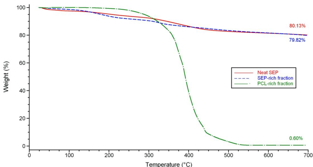
Figure 4.43: Weight loss curves of neat SEP, SEP-rich fraction and PCL-rich fraction of PCL/clay nanohybrid obtained from the polymerization catalyzed by CALB immobilized on sepiolite (SEPL3). TGA performed under air atmosphere.
