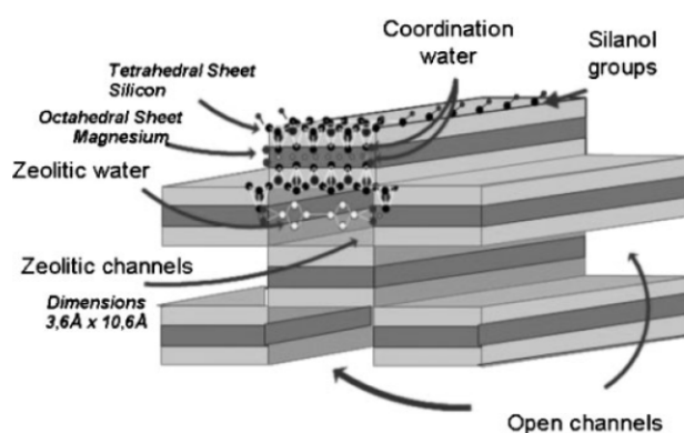
Figure 2.21 : Structure of sepiolite (Duquesne et al., 2007).
