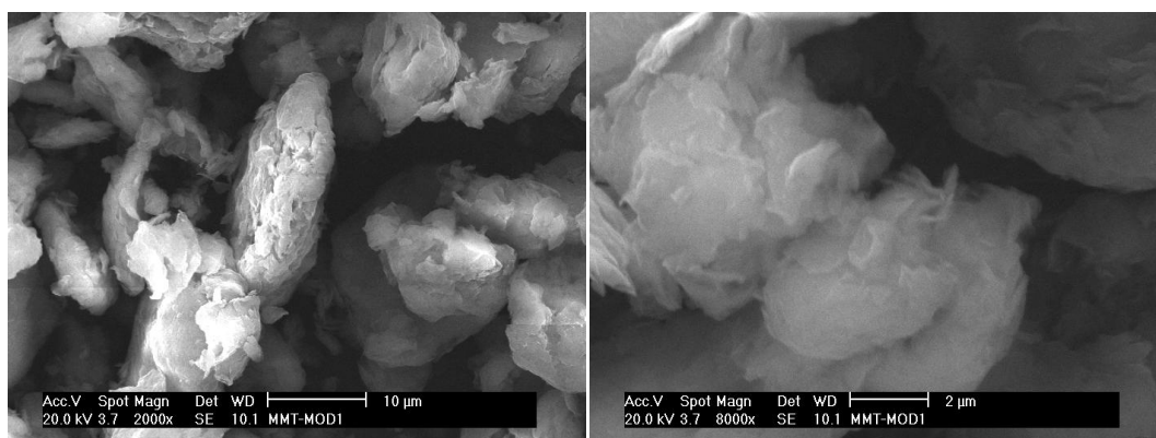
Figure 4.21 : SEM pictures of modified montmorillonite after immobilization of CALB (MMTMODL) at 2000x magnification (left) and 8000x magnification (right).
