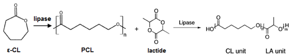
Figure 4.59 : Representation of a two steps copolymerization where PCL is firstly synthesized from \epsilon\text{-CL} by lipase catalysis followed by subsequent addition and polymerization of the lactide monomer.
