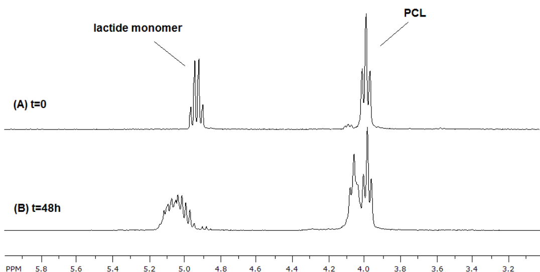
Figure 4.60 : Zoomed view of ^1\text{H} NMR spectra of samples (A) at t=0, where D lactide monomer is added to the reaction mixture containing the preformed PCL chain, (B) at t=48 h, final purified copolymer.
