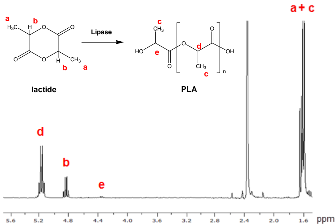
Figure 4.55 : Typical ^1\text{H} NMR spectrum of PLA synthesized by lipase catalyzed ROP of at 70\text{ }^\circ\text{C} . The proton assignments and corresponding peaks are shown in the spectrum.
