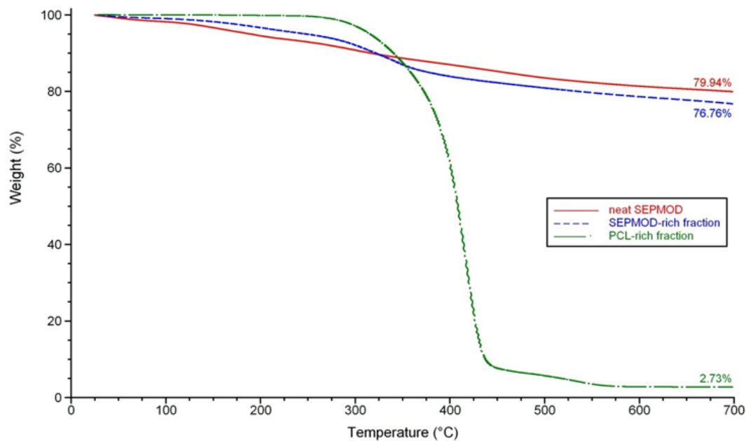
Figure 4.45 : Weight loss curves of neat modified SEP (SEPMOD), SEPMOD-rich fraction and PCL-rich fraction of PCL/clay nanohybrid obtained from the polymerization catalyzed by CALB immobilized on modified sepiolite (SEPMODL1G). TGA performed under air atmosphere.
