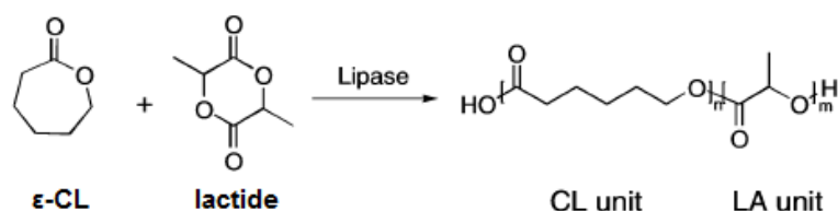
Figure 2.17 : Lipase catalyzed copolymerization of \epsilon -CL and lactide.
