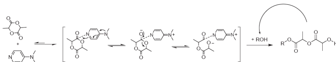
Figure 2.7 : Proposed mechanism for the ROP of lactide by DMAP.
