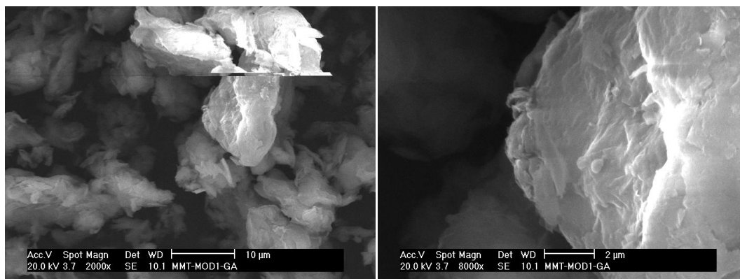
Figure 4.48 : SEM pictures of organo-modified montmorillonite after immobilization of CALB and treated with GA (MMTMODL G) at 2000x magnification (left) and 8000x magnification (right).
