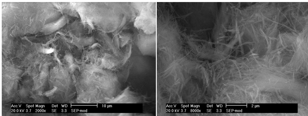
Figure 4.15 : SEM pictures of modified sepiolite (SEPMOD) at 2000x magnification (left) and 8000x magnification (right).
