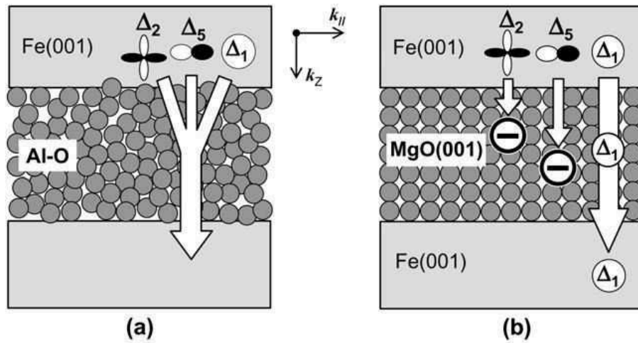
Figure 1.10: Schematic comparison of a) an incoherent tunneling through the Al_2O_3 amorphous barrier and b) a coherent transport through the crystalline MgO . [14].
