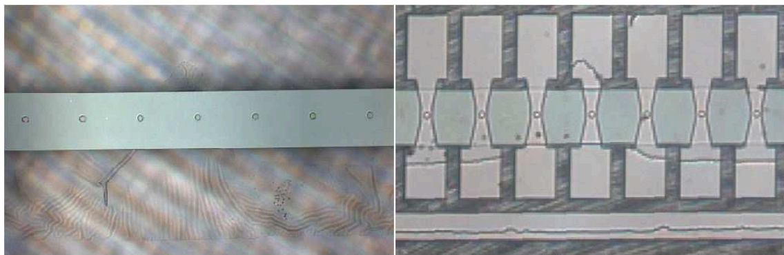
Figure 4.13: Left: Excessive lift-off of the passivation layer originating from the detouring edge causes its unwanted removal from the electrode area. Right: Impact of the phenomena on the final state of the sample. Lack of SiO 2 directly atop the junction in the middle and the one directly on its left causes short-circuiting of these devices as the current flows directly between the top and the bottom electrodes.
