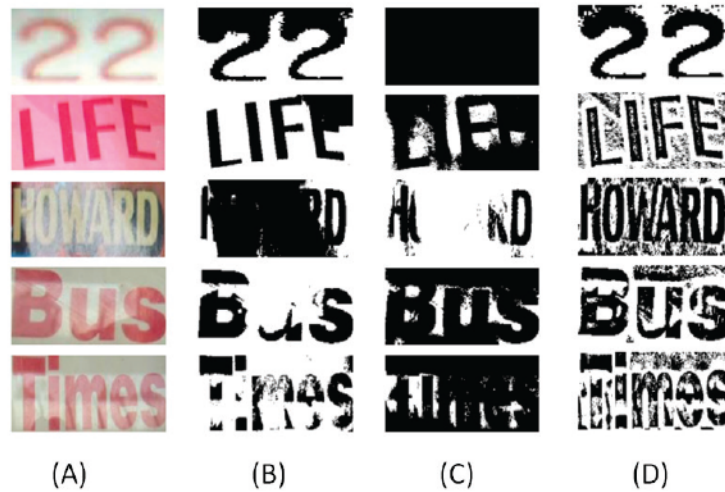
Figure 2.3: Comparison of some thresholding-based binarizations: (A) original text images, (B), (C) and (D) are respectively results of methods presented in [Ots75], [SSH97] and [Nib85] (figure provided by [MAJ11]).
