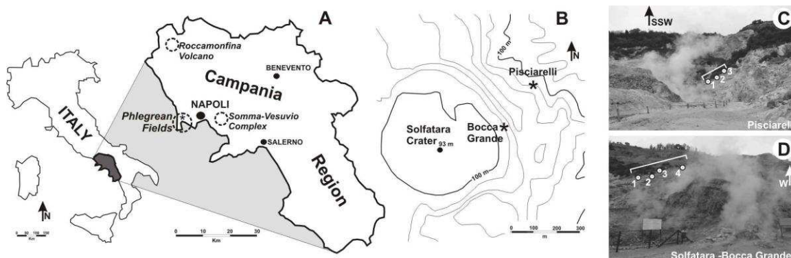
Fig. 1. (A) Location of the Phlegrean Fields and others gas-emitting volcanic areas (dotted circles) in Campania Region. (B) Sketch map showing the location of Solfatara crater and Pisciarelli locality. (C,D) Close up views of Pisciarelli and Solfatara localities with the main fumaroles. Square brackets indicate sampling areas and white circlets show the location of CO 2 measurements.
