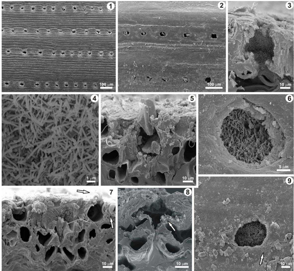
Plate I. Pinus halepensis , SEM of abaxial and adaxial cuticles, for to both trees experiencing and not chronic fumigation by volcanic gases. Stomatal class refers to Nicolotti et al. (2005) classification in which: class 0 = stomatal structure displaying no sign of alteration, class 1 = for slight sign of alteration, class 2 = for moderate sign of alteration, class 3 = for severe alterations.
