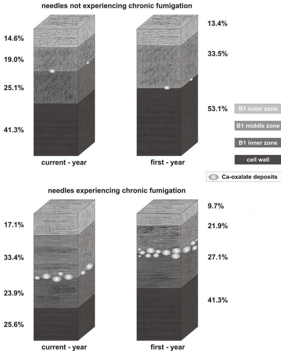
Fig. 5. Three-dimensional reconstruction of both cuticle and cell wall (CW) for needles experiencing- or- not chronic fumigation. Note: the cuticular membrane CM is made up with cuticular layer CL (= B = B1 divided in outer, middle and inner layers).
