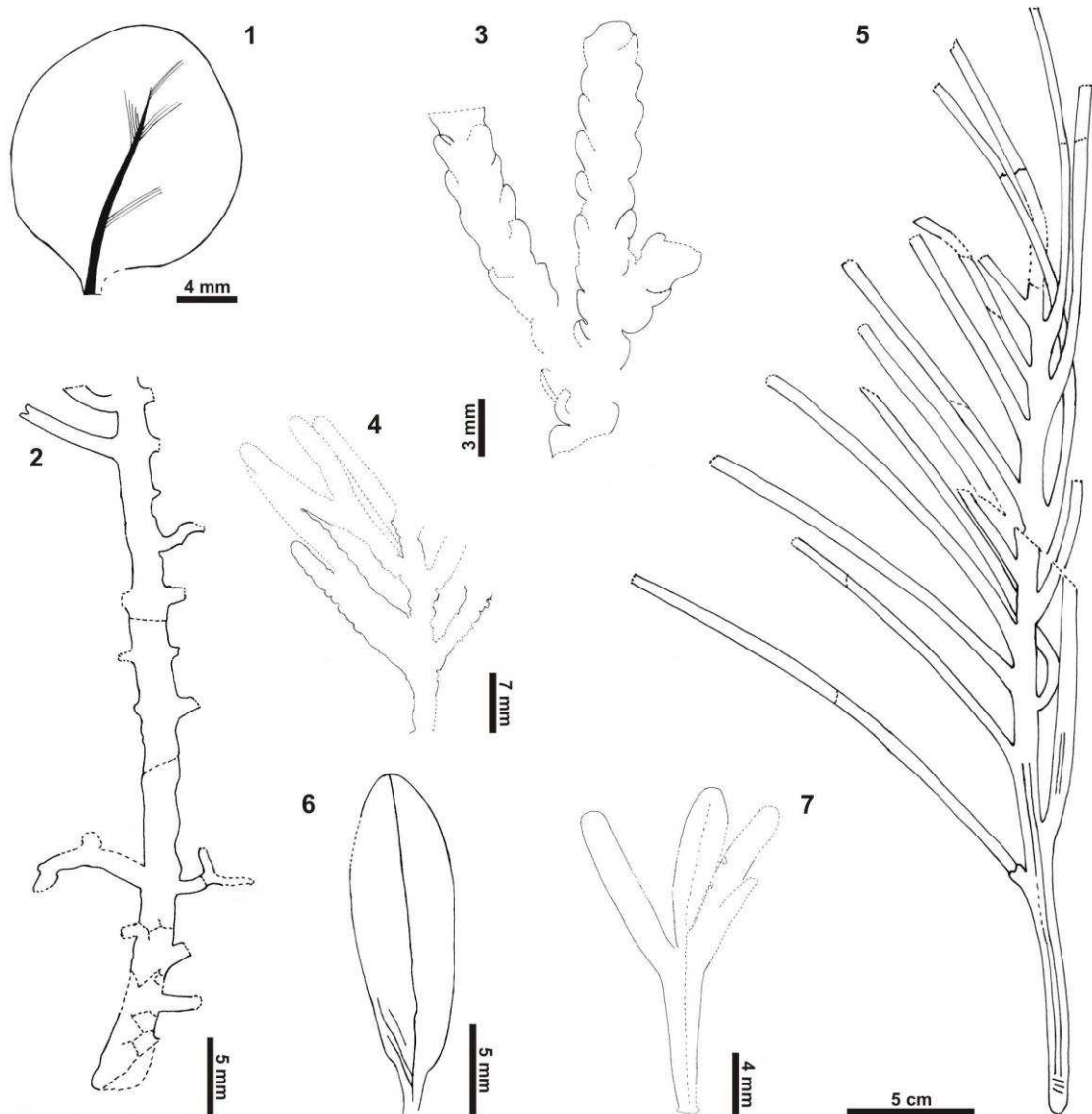
Fig. 3. Early Albian fossil plants from Pietraraja. Line drawings of selected specimens. 1. Sagenopteris? sp.. Showing primary and secondary veins (M 20802). 2. Brachyphyllum sp. 1. Showing branched specimen and poorly preserved leaf-scars in its basal part (M 20908). 3. Brachyphyllum sp. 2. Showing two-order branches and leaves tightly adpressed to the axis (M 20765). 4. Brachyphyllum sp. 2. Showing three-order branches (M 20909). 5. Frenelopsis sp.. Large branched specimen showing two-order branches and the central vascular bundle (M 20569). 6. Angiospermae 1. Showing the well-visible primary and secondary -in the basal part- veins (MF 1265). 7. Incertae sedis . Leaf showing three lobes and a distinct petiole (M 20796).
