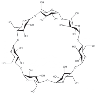
Figure 5: Representation of a \alpha -cyclodextrin molecule
