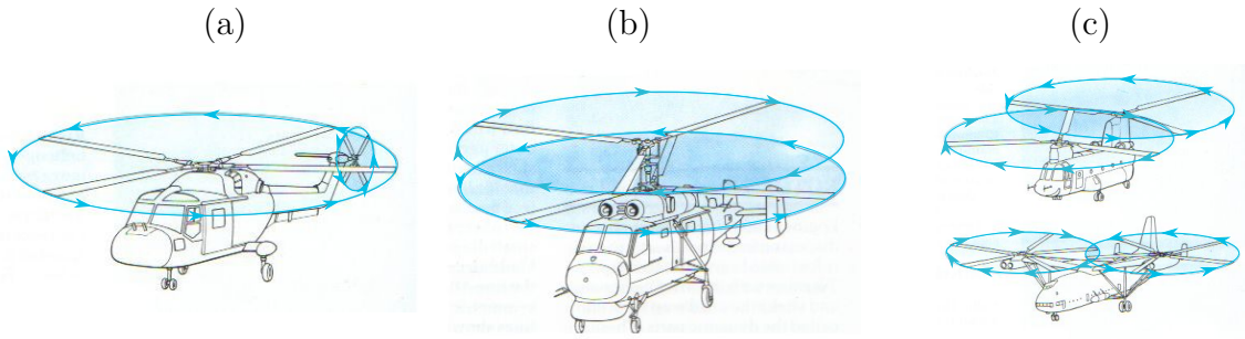
Figure 2.4: Different anti torque systems ( aerospaceweb.org ).
