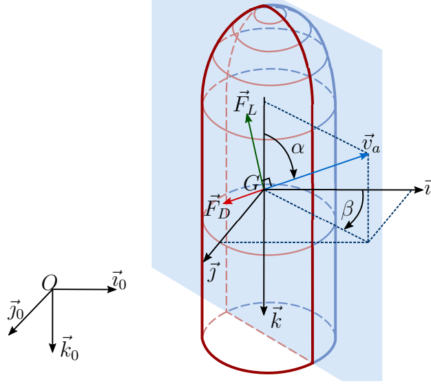
Figure 9.3: Aerodynamic forces and (\alpha, \beta) angles.
