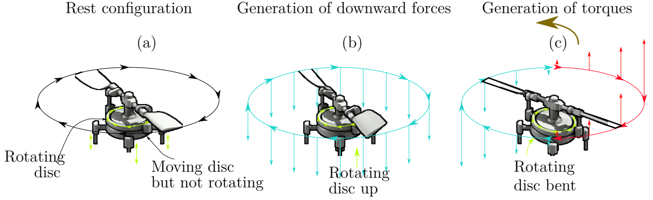
Figure 2.6: Effects of swashplate on the thrust force and torque produced by the blades.
