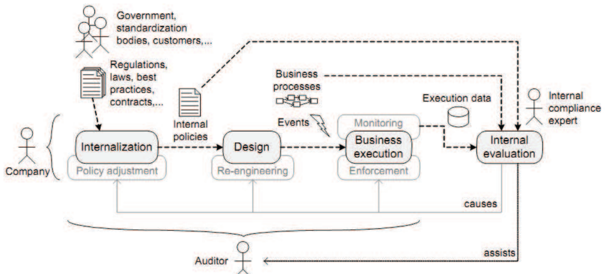
Figure 6: Compliance monitoring.
