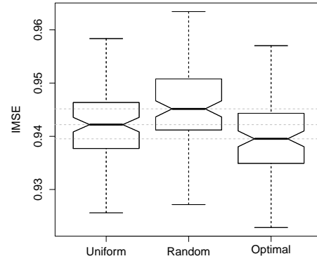
(b) d = 1, T = 50, n = 10, \theta = 5.10^{-3} k(\cdot, \cdot) : Gaussian, \eta(x) = \mu_U(x)
