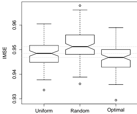
(c) d = 1, T = 50, n = 10, \theta = 5.10^{-3} k(\cdot, \cdot) : 5/2-Matérn, \eta(x) = \mu_U(x)
