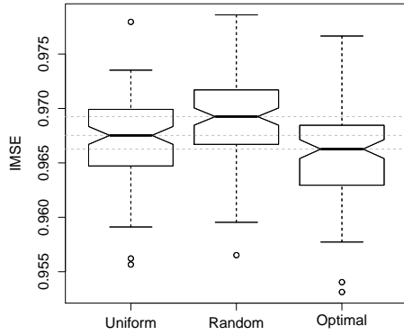
(a) d = 1, T = 50, n = 10, \theta = 5.10^{-3} k(\cdot, \cdot) : exponential, \eta(x) = \mu_U(x)
