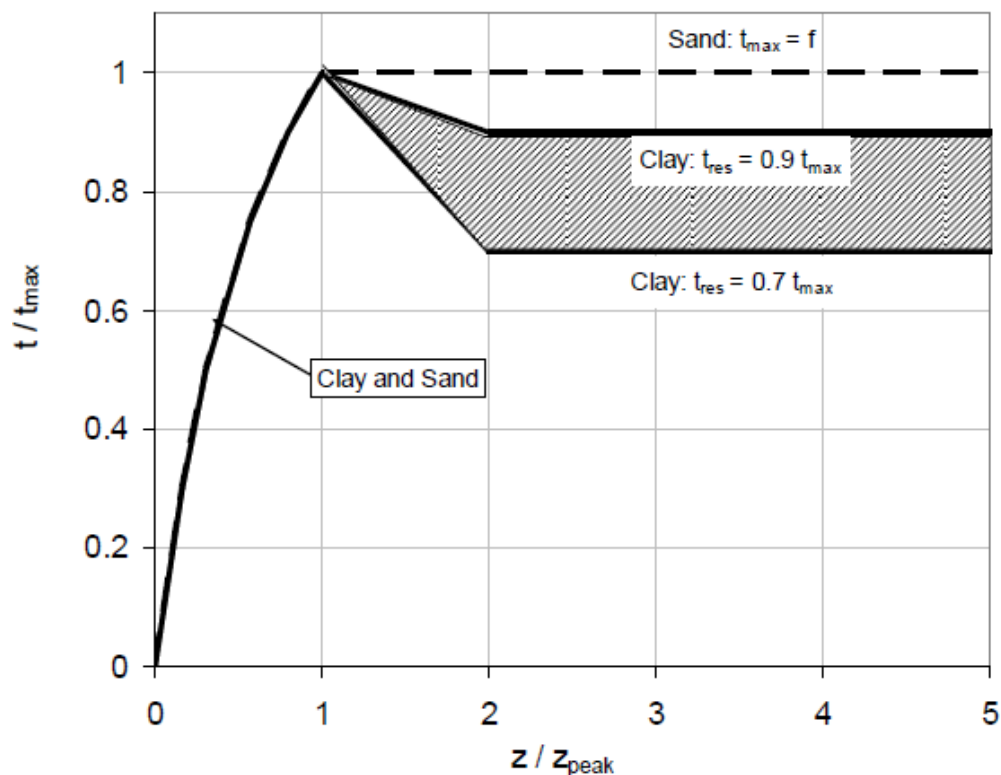
Figure I-13: Courbe T-Z (API RP 2GEO, 2011)
