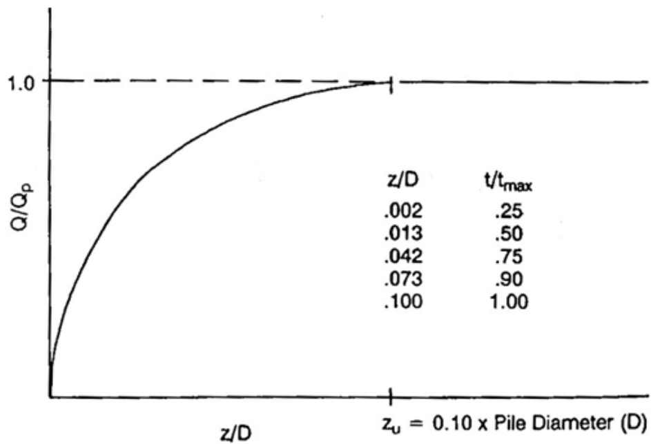
Figure I-14 : Courbe Q-Z (API RP 2GEO, 2011)
