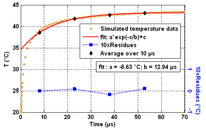
Fig. 11: results of the thermal transient simulation for the case of the EM4 photodiode, d = 32 \mu\text{m} , D = 450 \mu\text{m} , A = 152 \mu\text{m} (see geometry on Fig. 9), material conductivity 68 \text{ W m}^{-1} \text{ K}^{-1} and specific heat 0.31 \text{ J g}^{-1} \text{ K}^{-1} . Heat flux 112 \text{ W mm}^{-2} , corresponding to a Joule power of (6 \text{ mA}) \times (15 \text{ V}) . Note the \times 5 factor for the right scale (residues).
