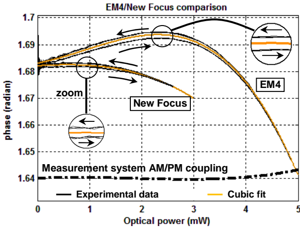
Fig. 2. RF phase versus optical power for the two photodiodes. Bias voltage: 15 V (EM4), 4.1 V (New Focus). Each data point has been averaged over 100 elementary data. The measurement channel optical power is scanned at a frequency of 3Hz. One of the two recordings has been translated so that the phase offsets coincide. The cubic fits (see Table II) apply to the middle of the up and down curves.
