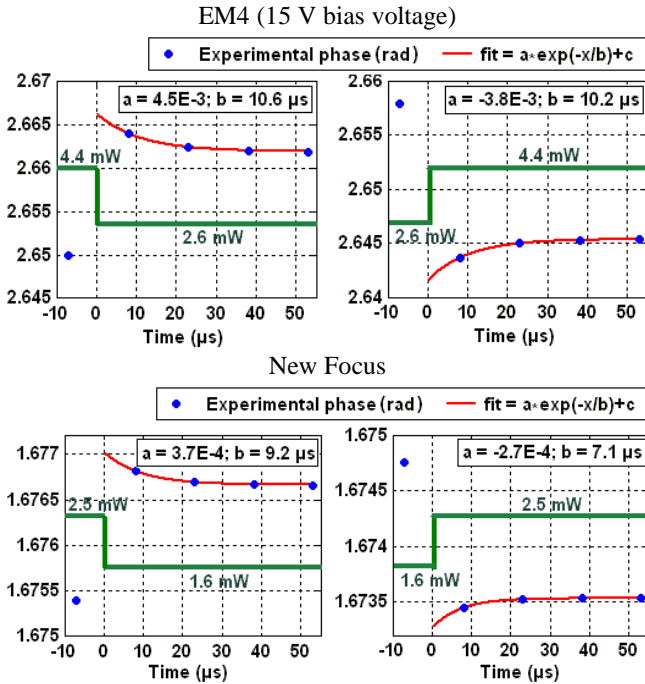
Fig. 8. Microsecond-scale transient behaviour of the phase after a sudden change of the optical power, for the two photodiodes under test. Data points are averaged over 4 \times 10^5 samples. Inset: values of the parameters of the exponential fit: amplitude (radians) and time constant ( \mu\text{s} ). Residues of the fit (RMS values) are of 1.2% and 0.4% for the EM4 and New Focus photodiodes, respectively.
