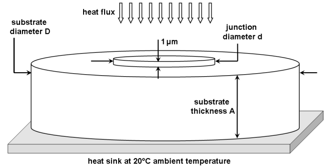
Fig. 10: Geometry of the junction/substrate/heat sink assembly used for the simulations. Drawing is not to scale.
