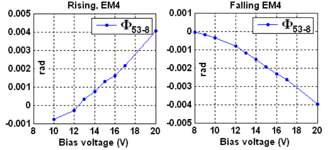
Fig. 9. Dependence of the amplitude of the short time ( \mu\text{s} ) transient behaviour of the phase, measured with the EM4 photodetector, as a function of the applied bias. The optical power is switched between 3.6 and 6.0 mW.
