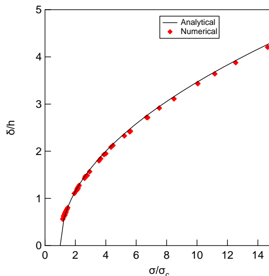
Figure 3.10: Out of plane displacement as a function of the loading ratio for numerical solution and analytical solution.
