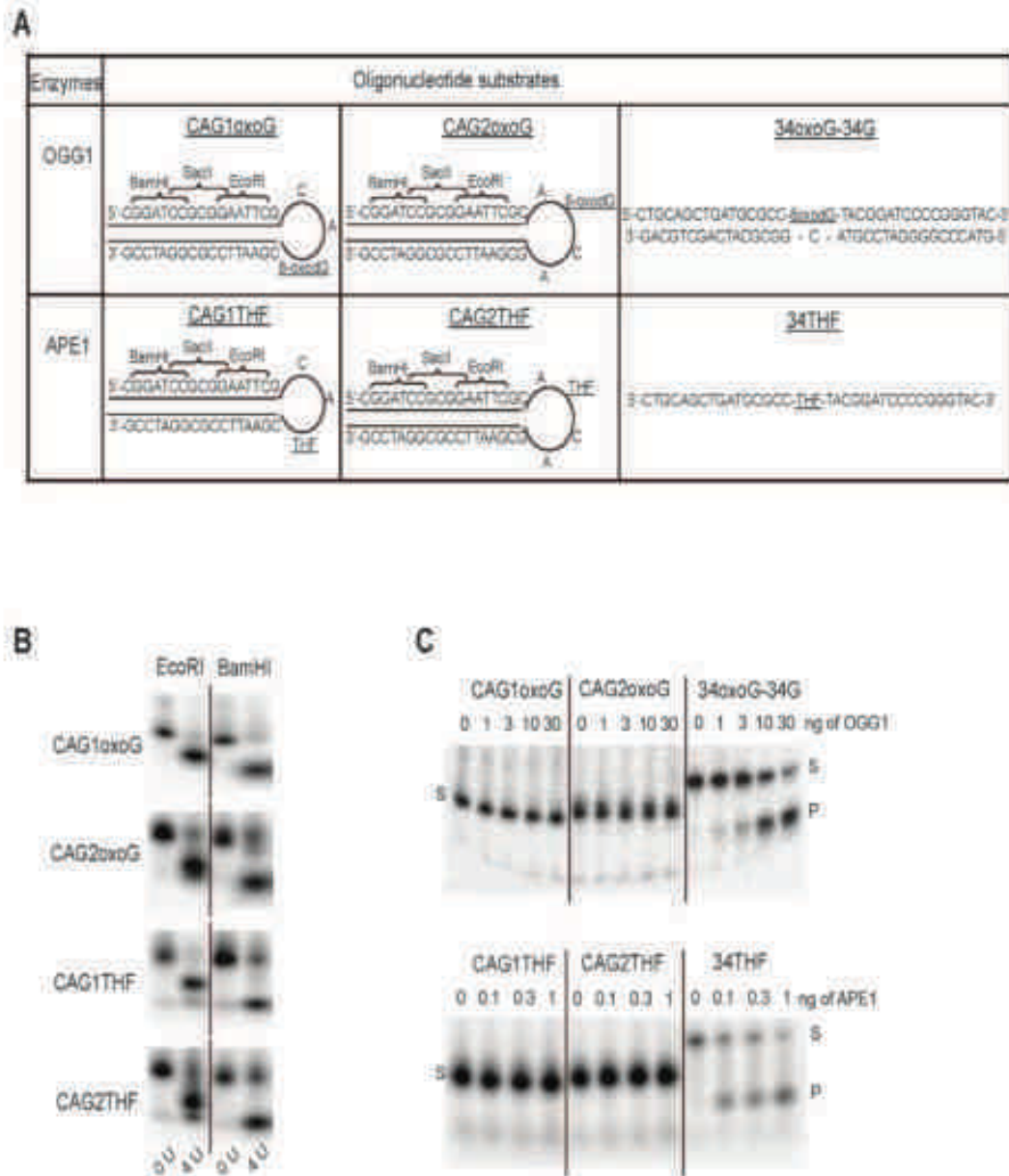
Figure 3. OGG1 and APE1 are unable to incise lesions at hairpin DNA structures. (A) Design of hairpin and control oligonucleotides. Hairpin oligonucleotides contain a 2-oxoG lesion or a THF lesion in 3-nt (CAG1oxoG or CAG1THF) or 4-nt (CAG2oxoG or CAG2THF) loop. The hairpin structured oligonucleotides contained BamHI, SacI and EcoRI restriction sites on the linear double stranded portion of the hairpin. (B) Digestion of hairpin oligonucleotides with EcoRI or BamHI (4 U). Efficient digestion shows that the designed oligonucleotides adopt a stable hairpin structure. (C) Hairpin and control oligonucleotides were incubated with increasing amounts of OGG1 (top panel) or APE1 (bottom panel). S: substrate, P: product. Recombinant enzymes efficiently incised control, but not hairpin, oligonucleotides.
