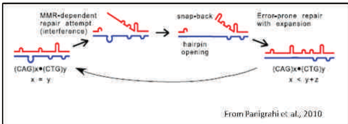
Figure 5. MMR and TNR instability model. CAG/CTG repeats form multiple slip-outs which may initiate repair process but lead to expansion product following error-prone repair. Some initiated repair could be arrested, leading to strand slippage, strand displacement and finally incorporation of structured repeats.
