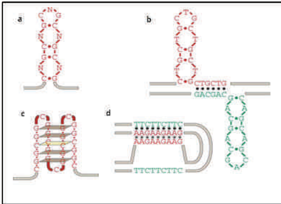
Figure 1. Unusual DNA structures formed by TNR repeats, examples.
