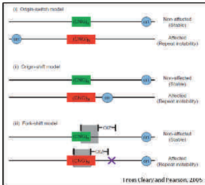
Figure 9: Current models implicating replication origin to the TNR instability. i) Origin-swift model: the replication origin orientation relative to the repeats suggests an influence on the repeat instability, ii) Origin-shift model: the distance of the origin replication relative to the repeats influences the repeats stability, iii) Fork-shift model: the presence of cis-elements (e.g. CTCF binding sites) between the replication origin and the repeats might influence repeat instability. (ori: replication origin, OIZ: Okazaki initiation zone) [Adapted by (Cleary and Pearson, 2005)]
