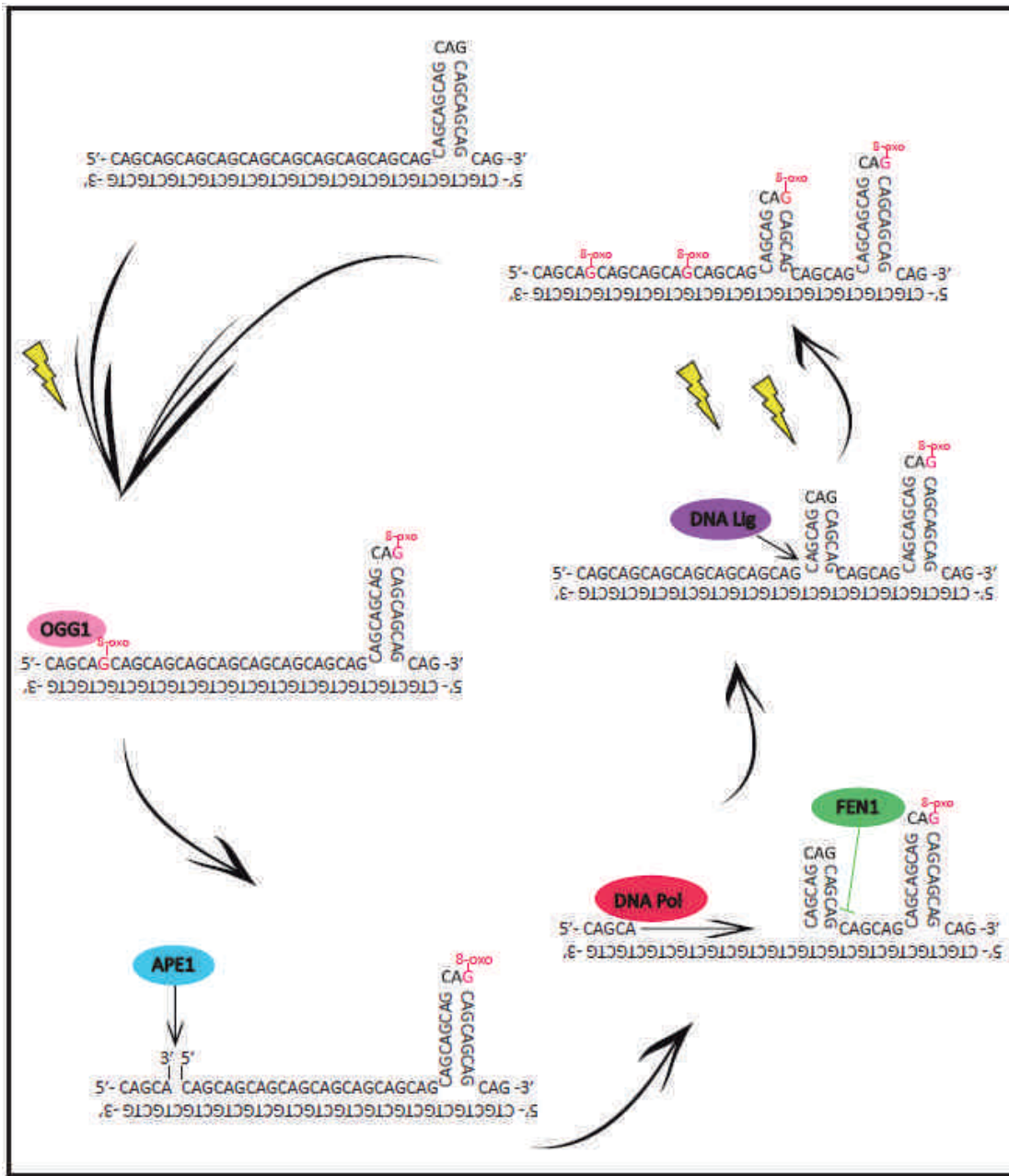
Figure 4. The “toxic oxidation cycle” model. An oxidant damage occurs at the CAG repeats and is processed by the BER machinery: a DNA glycosylase, e.g. OGG1, and APE1. A DNA polymerase due to strand displacement activity leads to incorporation of several nucleotides and adjacent to them to formation of a repeat hairpin –which can also be spontaneously formed. This hairpin structure is further stabilized by Msh2 and Msh3 complex and is refractory to excision from FEN1. DNA ligase I seals the nick leading to strand expansion. Oxidant damages are thought to increase with age leading to this error-prone repair and repeat instability.
