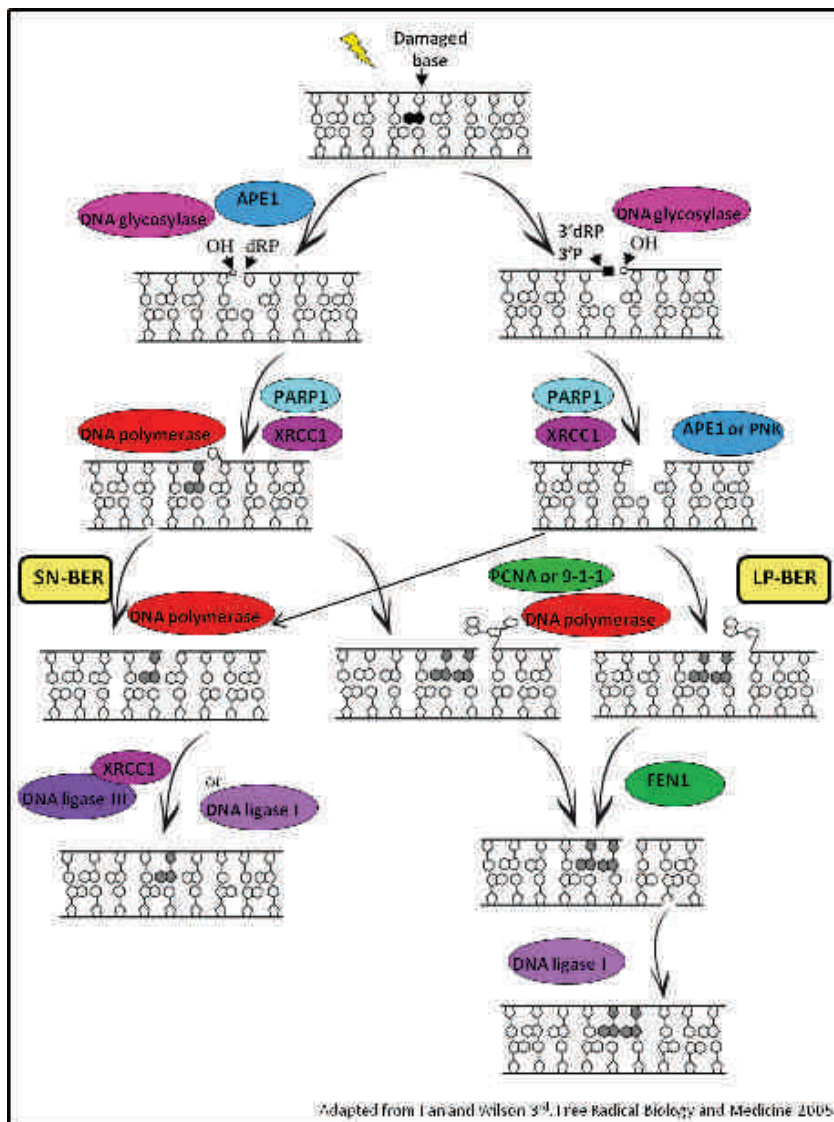
Figure 3. BER pathway and interplay between SN- and LP-BER. A DNA damage is excised by a monofunctional DNA glycosylase and APE1 leads to production of 3'OH and 5-dRP extremities. On the other site 3'dRP or 3'-phosphate (P) extremities generated by some bifunctional glycosylases, are processed by APE1 or PNK. In SN-BER a DNA polymerase incorporates 1 nucleotide and DNA ligase III/XRCC1 or DNA ligase I seals the nick. Addition of >1 nucleotide by DNA polymerase lead to formation of a 5'flappy strand excised by FEN1, in the case of LP-BER. Ligation of the nick is performed by DNA ligase I. PARP1 is a nick sensor, repair protein recruiter and coordinator; PCNA, 9-1-1 are repair proteins coordinators. [Adapted from (Fan and Wilson, 2005)]
