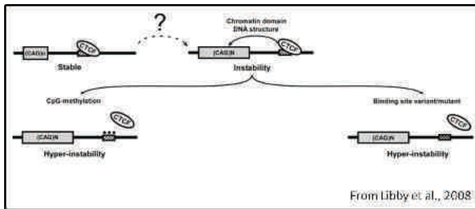
Figure 9. CTCF and TNR instability model. Binding of CTCF in its site protects CAG repeats from expansion. Once repeats expand, they alter the chromatin environment and DNA structure around them leading to instability. Loss of CTCF binding in its site following its mutation or CpG methylation leads to repeat instability, further suggesting that chromatin environment and repeats structures affect repeat instability.
