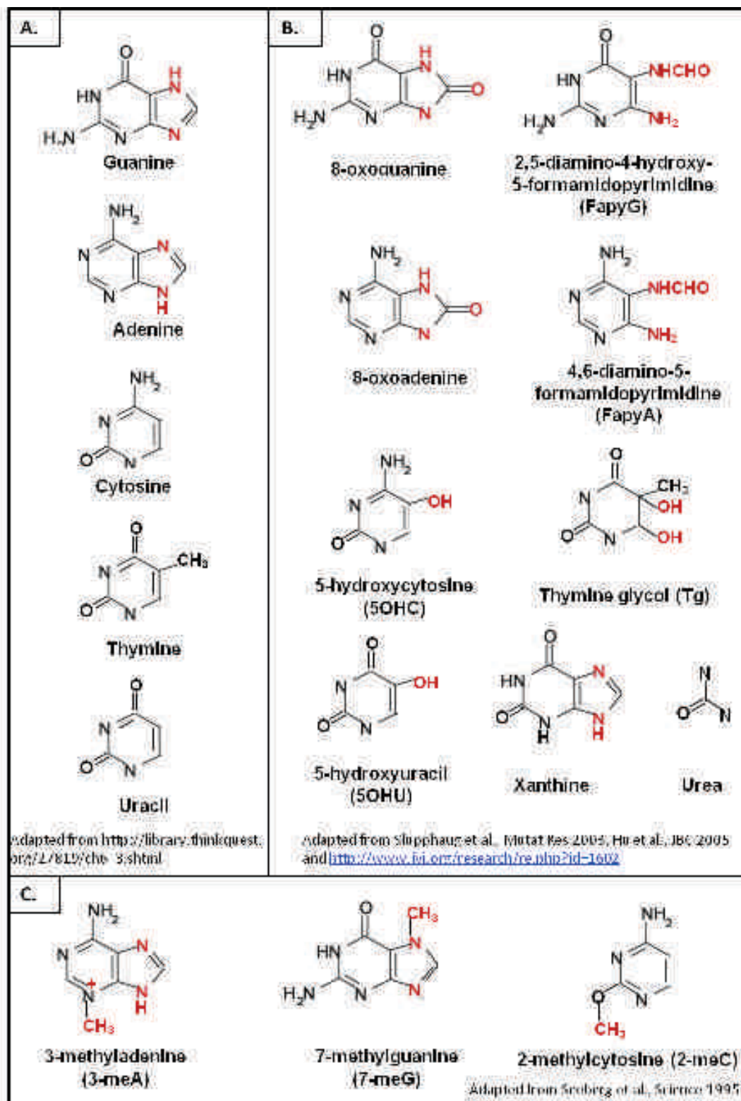
Figure 2. DNA bases and examples of common modifications. A. nucleic bases, B. common oxidized or reduced bases, C. common alkylated bases [Adapted by (Seeberg et al., 1995;
