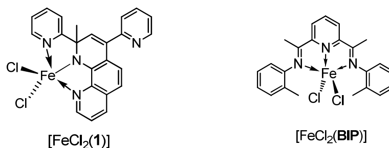
Scheme 3. Structures of complexes [\text{FeCl}_2(\mathbf{1})] (left) and [\text{FeCl}_2(\mathbf{BIP})] (right).
