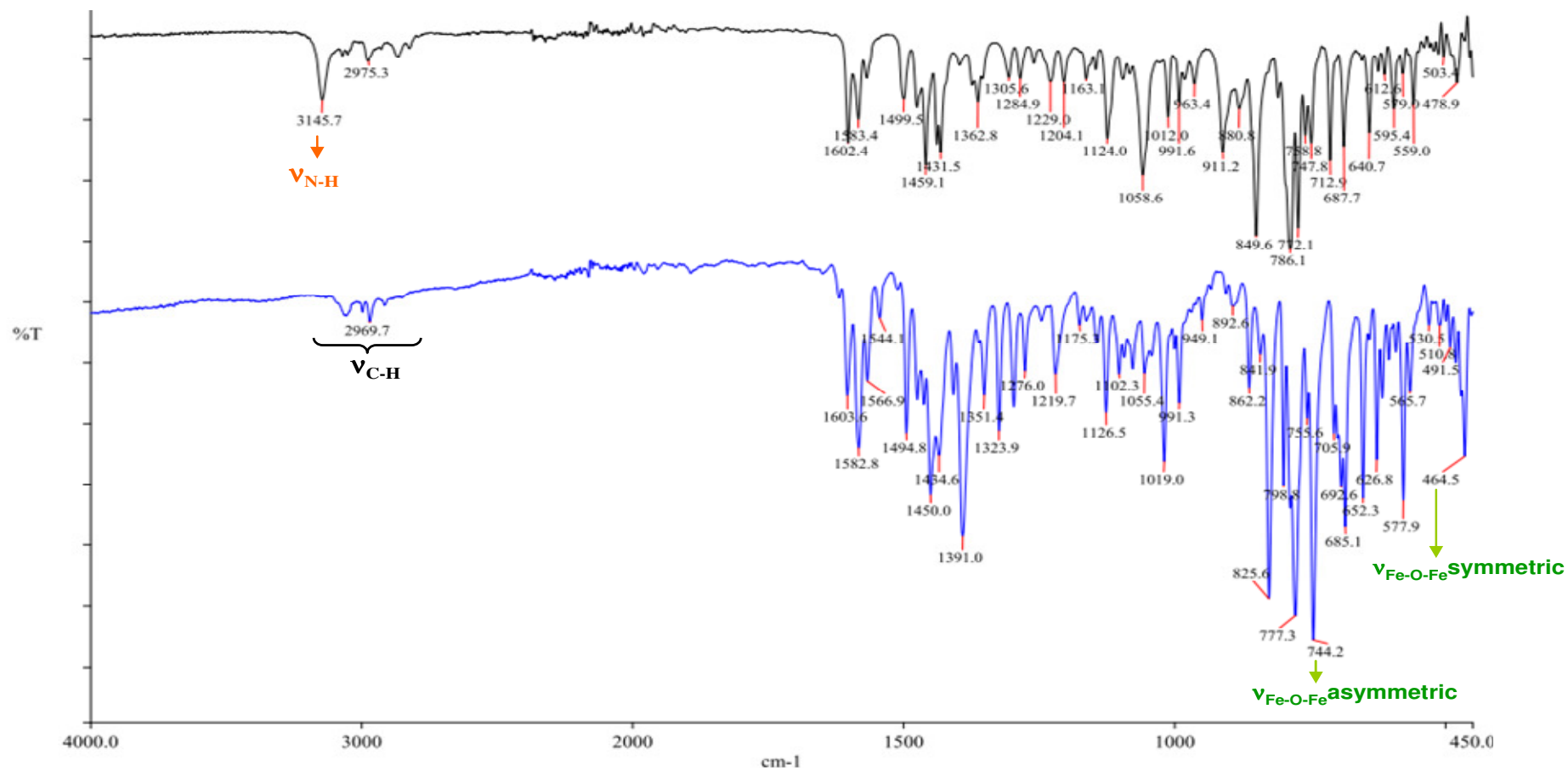
Figure 1. FT-IR spectra of the complex [\text{FeCl}_2(\text{H1})] (black) and the corresponding oxidized complex [(1)\text{FeCl}(\mu\text{-O})\text{FeCl}(1)] (blue)
