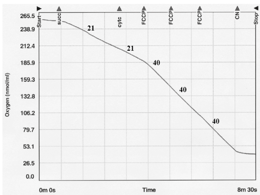
A.1 : Oxygen consumption of mitochondria isolated from a wild type strain. Representative plot illustrating oxygen consumption corresponding to 200µg of wild type mitochondria. Respiration rates are indicated in bold numbers for added chemical compounds. succ : succinate (10mM); cytc : cytochrome c (20µM); FCCP : carbonyl cyanide-4-(trifluoromethoxy)phenylhydrazone (5nM/addition); CN : potassium cyanide (2.5mM).
