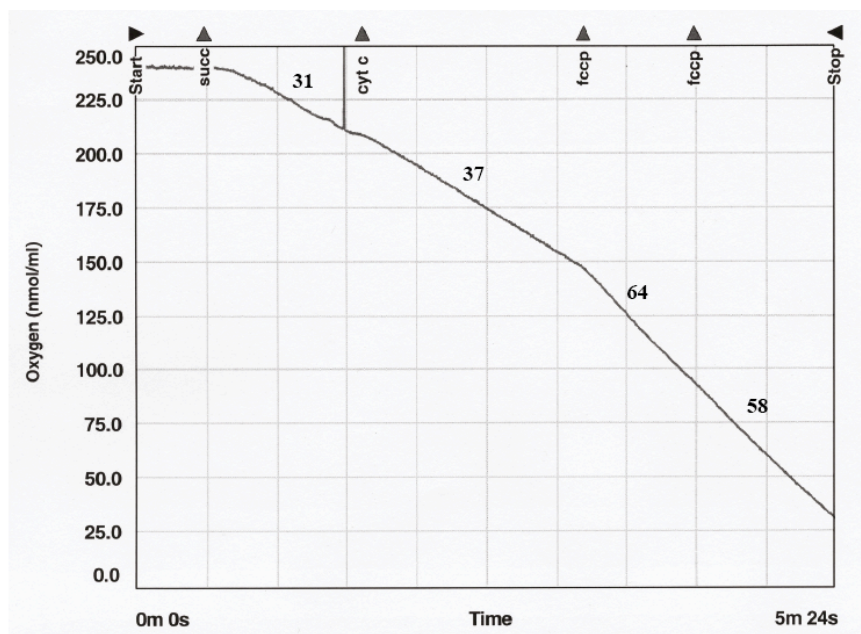
A.3 : Oxygen consumption of mitochondria isolated from a por2Δ strain. Representative plot illustrating oxygen consumption corresponding to 200μg of por2Δ mitochondria. Respiration rates are indicated in bold numbers for added chemical compounds. succ : succinate (10mM); cyt c : cytochrome c (12,5μM); FCCP : carbonyl cyanide-4-(trifluoromethoxy)phenylhydrazone (0,2nM/addition).
