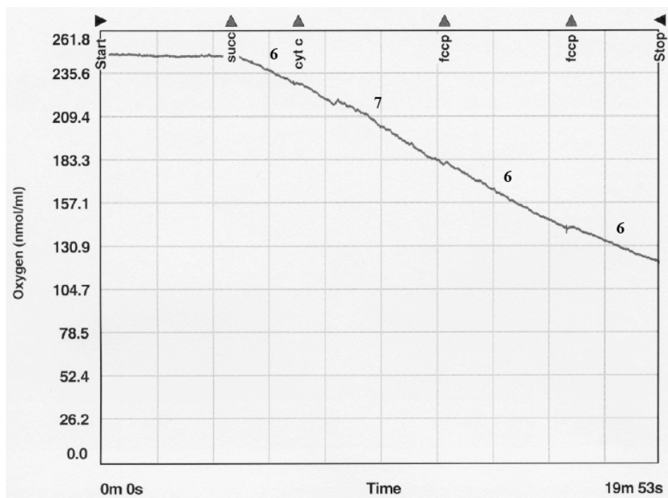
A.7 : Oxygen consumption of mitochondria isolated from a tom20 Δ 112 strain. Representative plot illustrating oxygen consumption corresponding to 200μg of tom20 Δ 112 mitochondria. Respiration rates are indicated in bold numbers for added chemical compounds. succ : succinate (10mM); cytc : cytochrome c (12.5μM); FCCP : carbonyl cyanide-4-(trifluoromethoxy)phenylhydrazone (5nM/addition).
