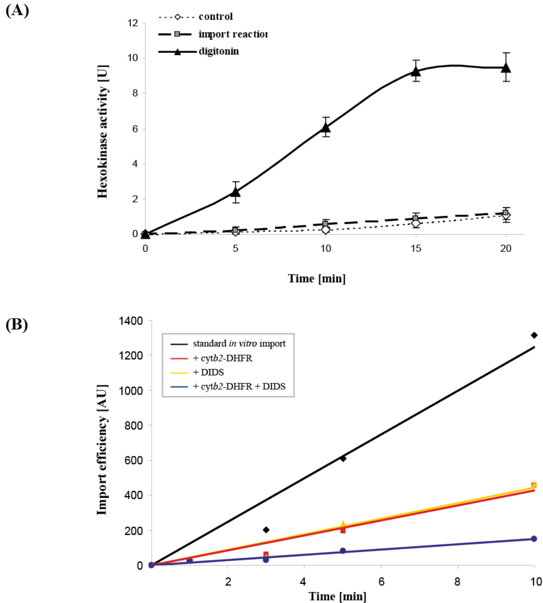
Fig.22 : Characterisation of outer membrane vesicles. (A) Outer membrane vesicles are stable in time at experimental conditions of in vitro tRK1 import. Amount of loaded hexkinase (HK) was checked by solubilising OMVs by digitonin and by measuring total HK activity in supernatant at indicated times after sedimentation of OMVs at 100000g. Leakiness of OMVs was investigated by measuring HK activity in supernatants of untreated OMVs (control) and in supernatants of OMVs in tRK1 in vitro import conditions in presence of tRK1 and import directing proteins enolase-2 and preMSK (import reaction). This graph is representative for OMVs derived from wild type mitochondria. HK activity [U] = \mu\text{mol} \cdot \text{min}^{-1} . (B) Linear character of time dependant in vitro tRK1 import into OMVs. tRK1 import kinetics was monitored by autoradiography and tRK1 import was quantified as explained in material and methods. Used colors: black for standard tRK1 in vitro import reaction; red for tRK1 in vitro import reaction into OMVs pre-treated with cytb2-DHFR; yellow for tRK1 in vitro import reaction into OMVs pre-treated with 1mM DIDS and blue for tRK1 in vitro import reaction into OMVs pre-treated with cytb2-DHFR and DIDS. [AU] = Arbitrary unit.
