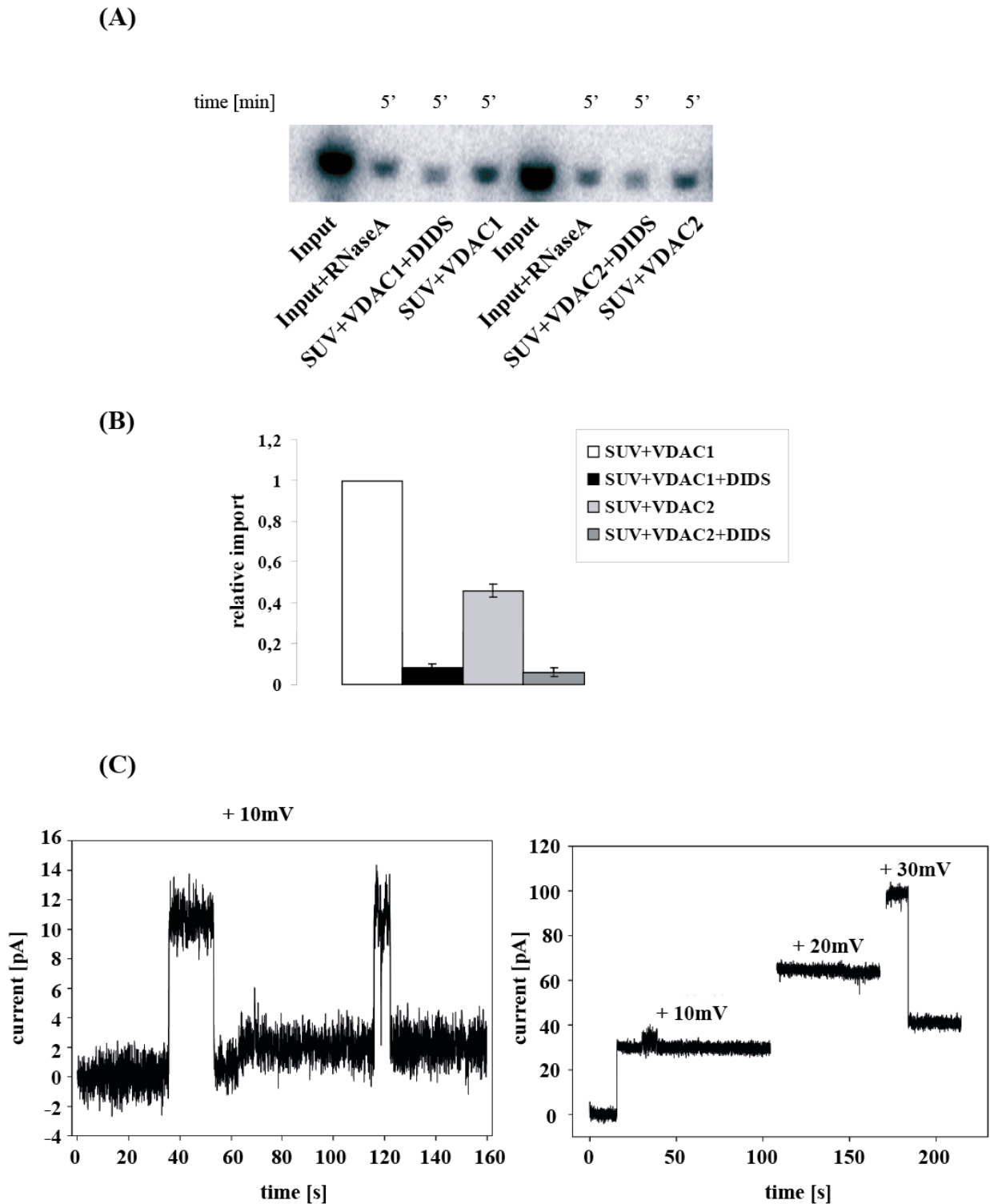
Fig.26 : In vitro of tRK1 into small unilamellar vesicles (SUVs) reconstituted with VDAC1 or VDAC2. (A) Autoradiogram illustrating in vitro tRK1 import into SUVs reconstituted with VDAC1 or VDAC2 in presence or absence of DIDS (0,25mM). Imports were performed in 100 \mu l SUV solution containing 0,1 \mu g of reconstituted protein. (B) Plot illustrating in vitro import of tRK1 into SUVs (import into SUV+VDAC1 was set to 1). (C) Voltage dependent conductivity of VDAC2 channels in presence of 1M KCl. left panel : channel recording performed with an applied potential of +10mV. right panel : channel recording performed at applied voltages of +10mV, +20mV and +30mV.
