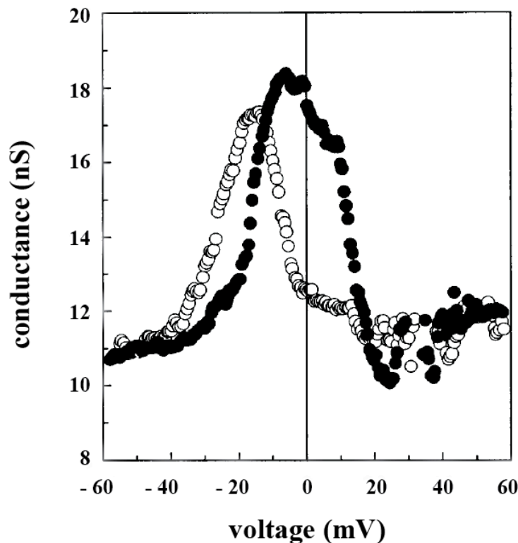
Fig.3 : Bell-shaped voltage dependance of VDAC conductance. In presence of an ATP gradient maximal channel conductance is observed between -15mV and -10mV. Higher potential values induce partial closure of the channels. ● Voltage change from negative to positive values. ○ Voltage change from positive to negative values (Rostovsteva et al., 1997).
