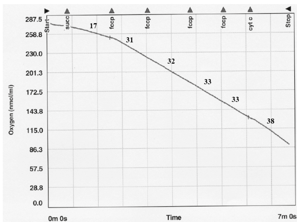
A.6 : Oxygen consumption of mitochondria isolated from a tom7Δ strain. Representative plot illustrating oxygen consumption corresponding to 200μg of tom7Δ mitochondria. Respiration rates are indicated in bold numbers for added chemical compounds. succ : succinate (5mM); cytc : cytochrome c (6μM); FCCP : carbonyl cyanide-4-(trifluoromethoxy)phenylhydrazone (5nM/addition).
