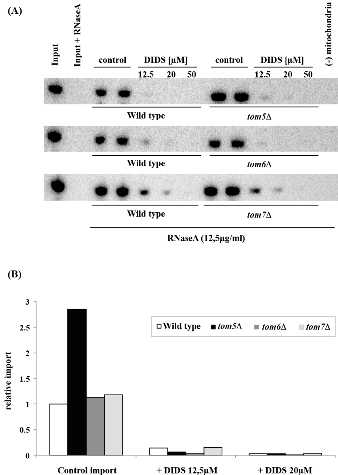
Fig.31 : Impact of the TOM complex stability on in vitro tRK1 import into isolated mitochondria. (A) Autoradiogram illustrating tRK1 import into isolated mitochondria of wild type (WT), tom5 \Delta , tom6 \Delta and tom7 \Delta S.cerevisiae strains in absence or presence of DIDS. Import reactions were performed for 5 minutes. (B) Plot illustrating relative tRK1 import into mitochondria of different S.cerevisiae strains (control import into WT mitochondria was set to 1 for each independent experiment).
