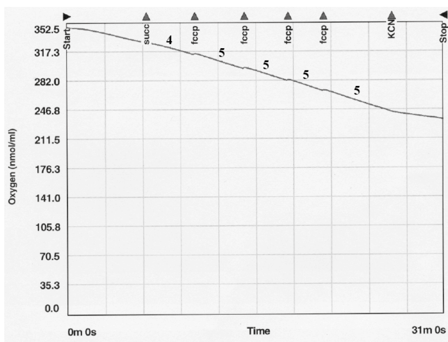
A.2 : Oxygen consumption of mitochondria isolated from a por1Δ strain. Representative plot illustrating oxygen consumption corresponding to 500µg of por1Δ mitochondria. Respiration rates are indicated in bold numbers for added chemical compounds. succ : succinate (10mM); FCCP : carbonyl cyanide-4-(trifluoromethoxy)phenylhydrazone (10nM/addition); CN : potassium cyanide (2mM).
