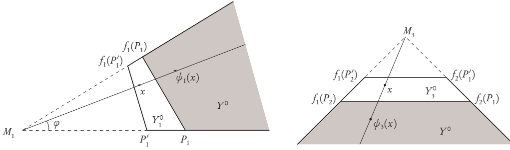
Figure 3.6: Left: Construction of the mapping \xi_1 : Y_1^0 \rightarrow Y^0 . Right: Construction of the mapping \xi_3 : Y_3^0 \rightarrow Y^0 .
