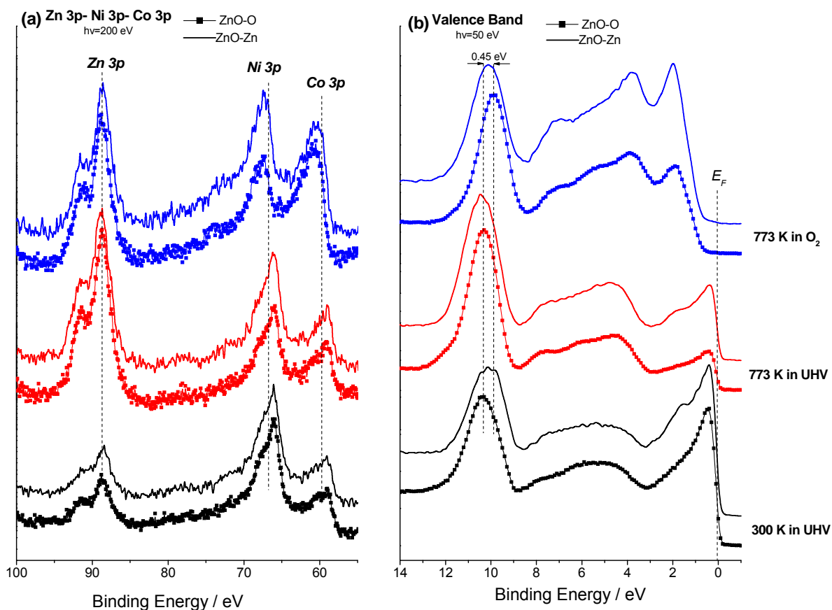
Figure 4.5. Zn, Ni, Co3p core-level (a) and valence band (b) spectra of 1.5 nm Ni-Co layer on ZnO-Zn(—) and ZnO-O(■) substrates as deposited (bottom), annealed at 773 K in UHV (middle) and after 1 \times 10^{-6} mbar O 2 at 773 K (top).
