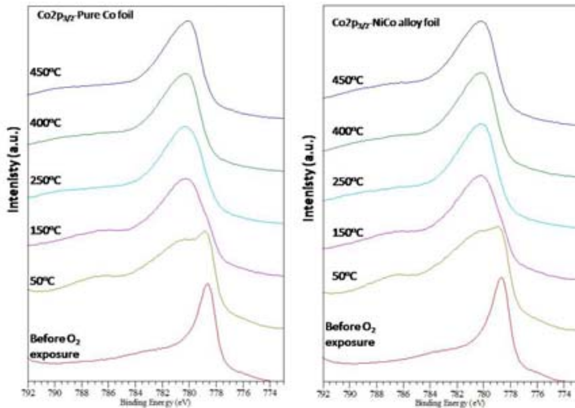
Figure 1.2 (Left) Normalised XPS spectra of Co2p_{3/2} for Co metal foil exposed to O 2 at 0.5bar (Right) Normalised XPS spectra of Co2p_{3/2} for NiCo alloy foil exposed to O 2 at 0.5bar. The time of O 2 exposure is 5 minutes for temperature 50°C, 150°C, 250°C, 400°C and 450°C
