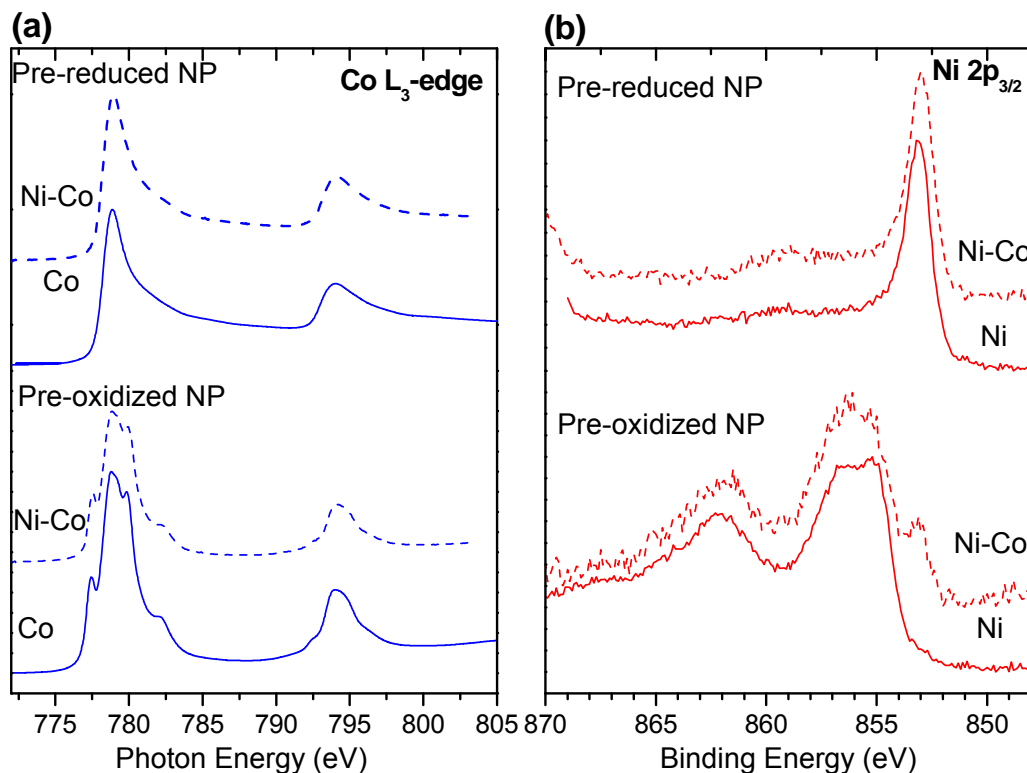
Figure 6.4 (a) Co L 3 edge of pre-oxidized (O 2 , 543 K) and pre-reduced (H 2 , 543 K) Co nanopowder (NP) and Ni-Co NP (b) Ni 2p 3/2 spectra of Ni NP and Ni-Co NP in ESR reaction gas mixture (ethanol to steam ratio=1:3) at 543 K.
