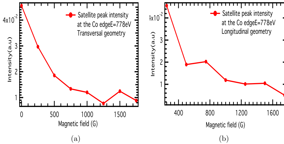
Figure 6.28: (a) Intensity of the satellite peaks in function of the applied magnetic field for the (a) Transverse configuration and (b) Longitudinal configuration.
