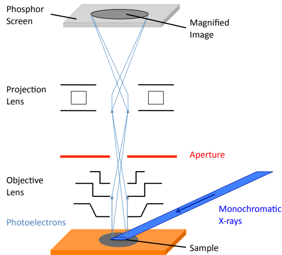
Figure 6.35: Sketch of a PEEM microscope
