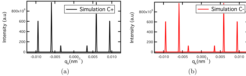
Figure 6.25: Polar simulations of the satellites with (a) right ( C^+ ) and (b) left ( C^- ) circular polarizations.
