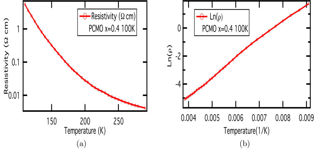
Figure 7.7: Resistivity curves of PCMO x=0.4 sample. No sign of a CO transition at T=220\text{K} or 1/T=0.0045\text{ K}^{-1} is observed
