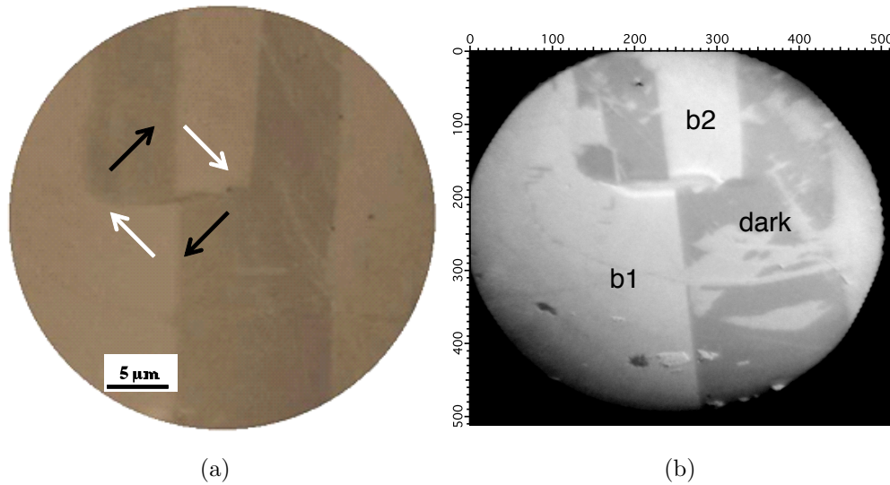
Figure 6.37: (a)Optical PLM image of FE multidomain BFO. (b)XLD X-PEEM image of FE multidomain BFO
