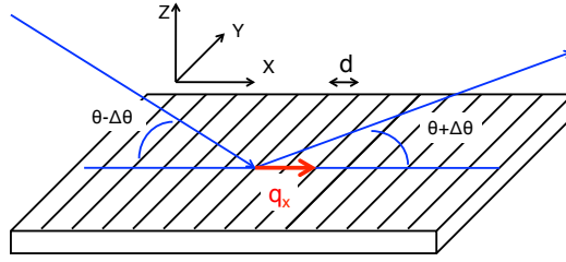
Figure 6.7: Rocking curve geometry. The detector is fixed at 2\theta = 2 \times \theta . The sample is turned around the Y axis from -\Delta\theta to +\Delta\theta .
