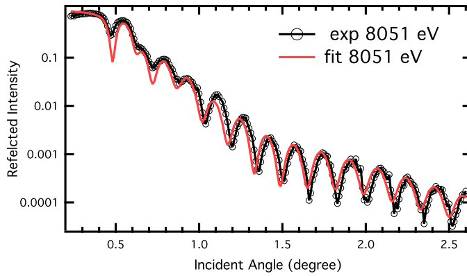
Figure 4.5: Experimental (symbols) and calculated (solid line) specular reflectivity for W/Fe/W at 8051 eV
