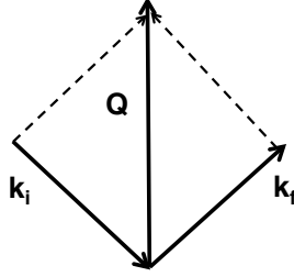
Figure 3.1: Diffraction vector
