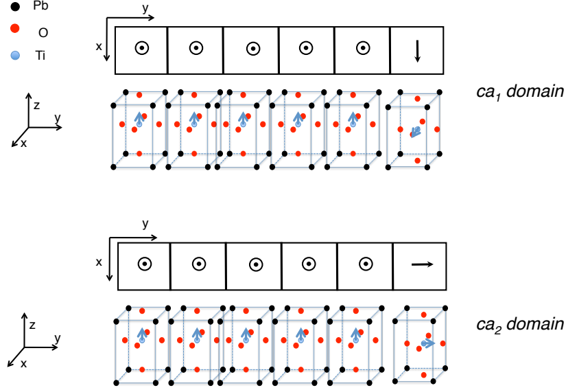
Figure 5.17: An example of two different patterns of unit cells which were used as input for the calculation of domain reflections
