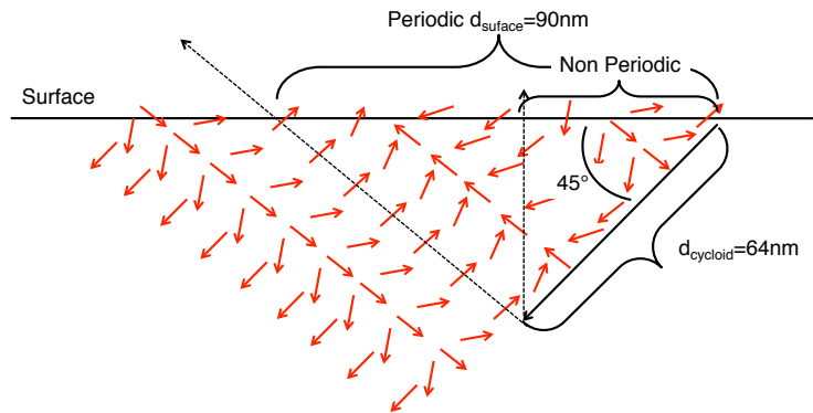
Figure 6.6: The projection of a cycloid on the surface plane of the sample. The periodicity on the surface is d_{surface} = d_{cycloid} / \cos 45^\circ with d_{cycloid} = 64 \text{ nm}
