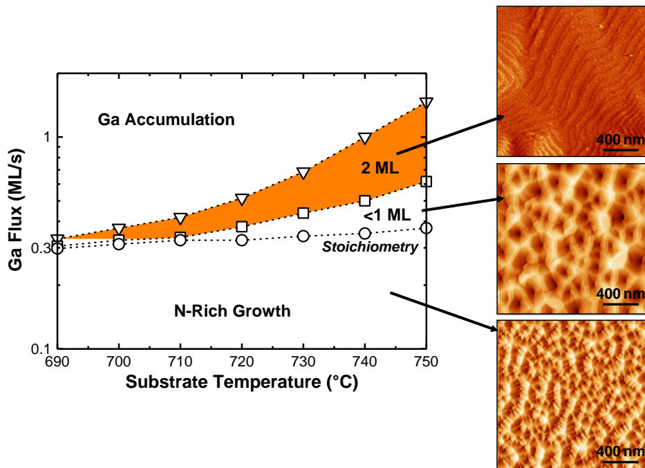
Figure 3.11. Ga coverage regimes as a function of both substrate temperature and impinging Ga flux.
