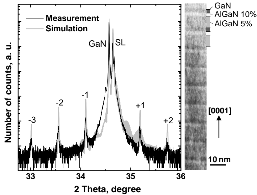
Figure 7.5. High-resolution \omega - 2\theta scan around (0002) x-ray reflection of step QW SL (black) and theoretical calculations (gray) using X'Pert Epitaxy 40 software from Philips Analytical. On the right is the cross-section conventional transmission electron microscopy image of the active region of the sample. The image contrast qualitatively correlates with the chemical composition of the layers.
