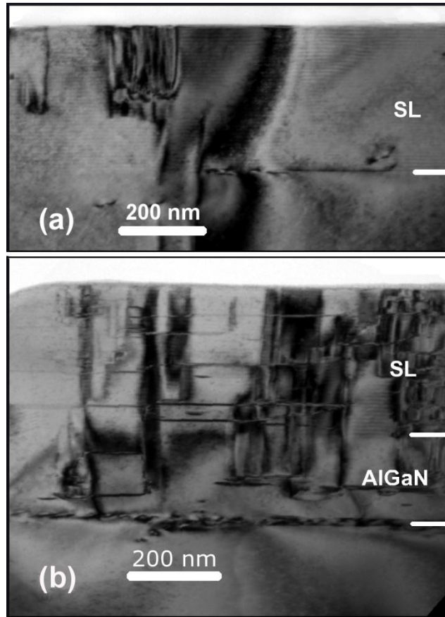
Figure 4.7. Two-beam TEM images of GaN/Al 0.3 Ga 0.7 N SLs deposited (a) on GaN and (b) on Al 0.3 Ga 0.7 N, viewed along the \langle 1-100 \rangle zone axis with diffraction vector g = (11-20) .
