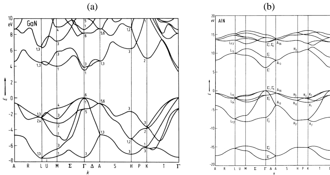
Figure 2.4. Band structure of (a) GaN (Bloom, 1974) and (b) AlN (Kobayashi, 1983).
