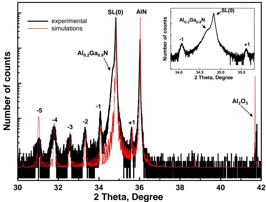
Figure 6.13. X-ray \theta - 2\theta scan of the (0002) reflection (black) for the QCD B (E2682). The insert is the zoom of the superimposed SL and buffer layers peaks. The superimposed thinner simulations (red) were performed using the program X'Pert Epitaxy 4.0 from Phillips Analytical.
