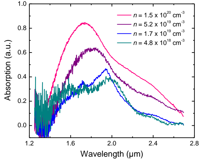
Figure 5.9. Infrared absorption spectra for TM-polarized light measured from GaN / AlN (2 nm/3 nm) QWs of series A grown on GaN-on-sapphire templates.
