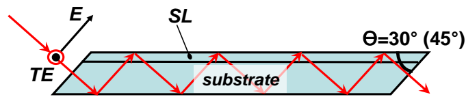
Figure 3.22. Waveguide multipass geometry for ISB measurements.
