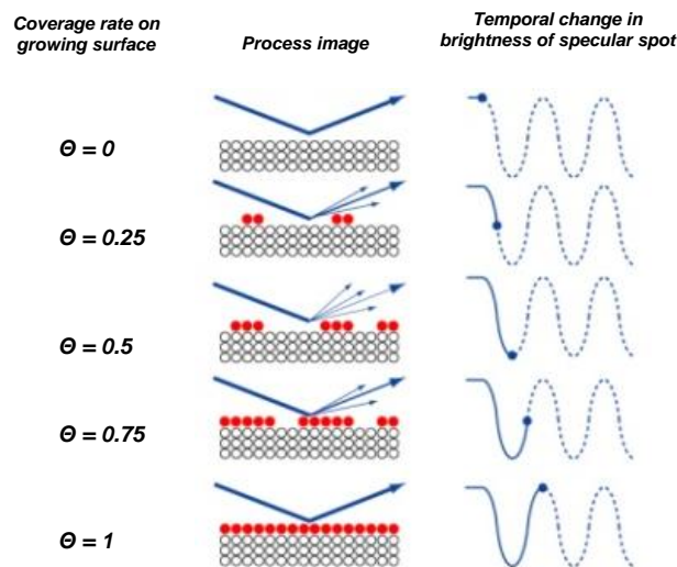
Figure 3.4. RHEED oscillation during the epilayer deposition.
