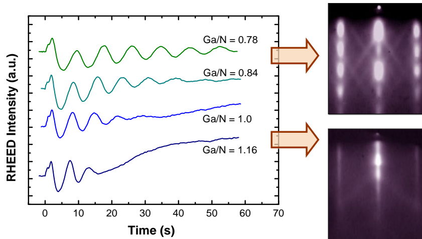
Figure 3.8. RHEED intensity oscillations and pattern at different III/V ratios.
