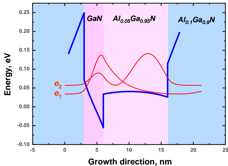
Figure 7.3. Conduction band profile and envelope functions of a GaN/ \text{Al}_{0.05}\text{Ga}_{0.95}\text{N} / \text{Al}_{0.1}\text{Ga}_{0.9}\text{N} step QW within a superlattice.
