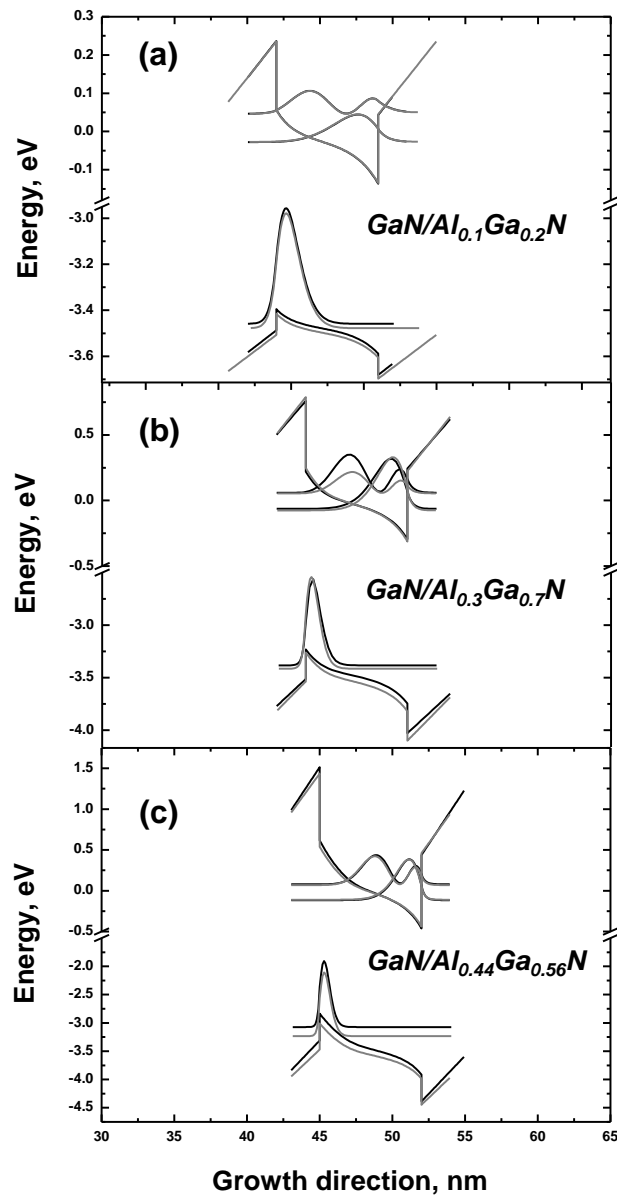
Figure 4.1. Conduction band profile and squared envelope functions of QWs in GaN/Al x Ga 1-x N (7 nm/4 nm) SLs with (a) x = 0.1 , (b) x = 0.3 , (c) x = 0.44 . Black (red) lines describe the structures fully strained on Al x Ga 1-x N (GaN).
