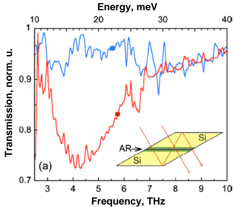
Figure 7.6. Transmission spectra for TM- (red) and TE-polarized (blue) light at 4.7 K for a step-QW SL. The inset shows the experimental configuration with two pieces face-to-face and the ray tracing. The active region is shown by an arrow.
