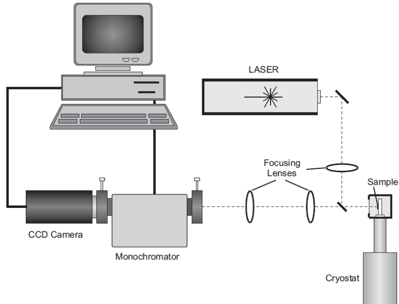
Figure 3.15. Photoluminescence setup.
