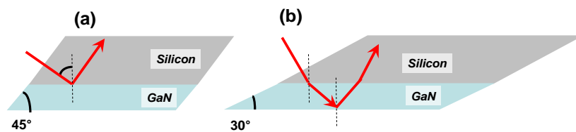
Figure 3.23. Multipass waveguiding geometry of HEMT-on-Si template with two facets polished at (a) 45° and (b) 30°.
