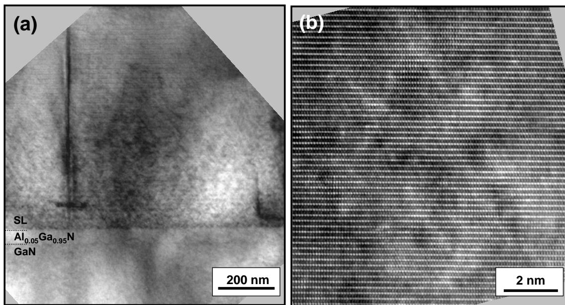
Figure 7.4. (a) TEM and (b) high-resolution TEM images of a step QW SL.
