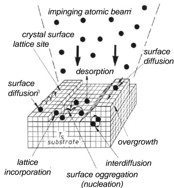
Figure 3.5. Schematic illustration of the main surface processes during MBE growth (Hermann, 1986).
