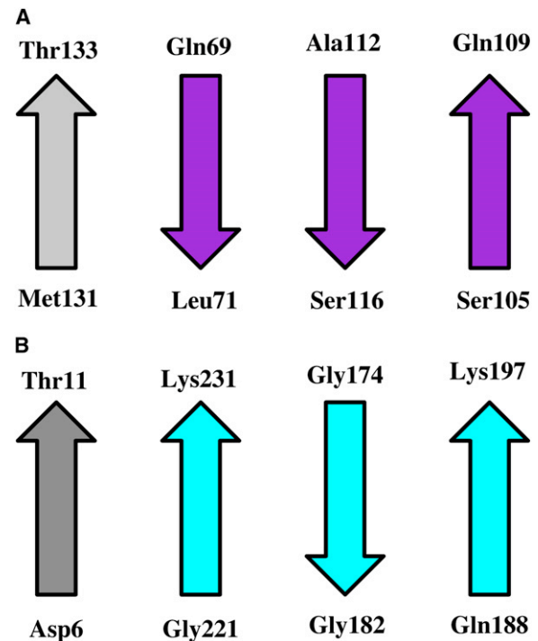
Figure 6. The \beta Strand Lock Exchange
