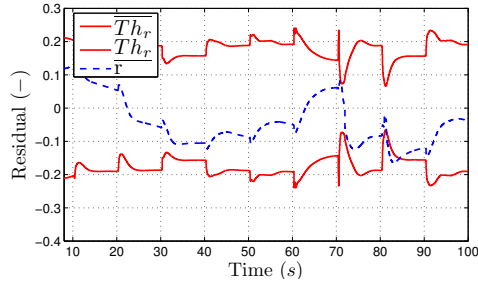
(c) Low Load, \Delta\eta_t = 0 , \Delta p_{exh} = 200\text{mbar}
