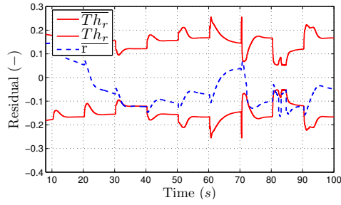
(e) Low Load, \Delta\eta_t = -10\% , \Delta p_{exh} = 200\text{mbar}
