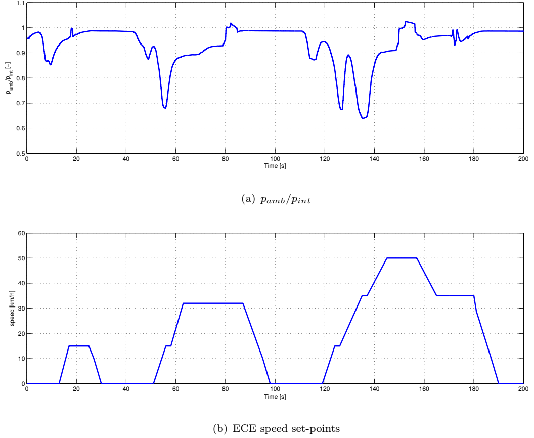
Figure 3.2: The observability condition measured along a urban driving cycle - ECE.
