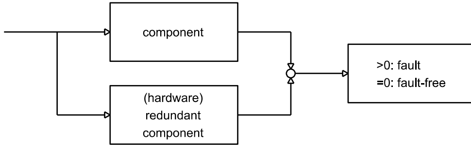
Figure 1.3: Hardware redundancy fault detection scheme
