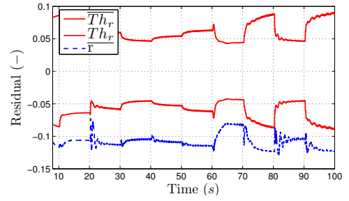
(f) High Load, \Delta\eta_t = -10\% , \Delta p_{exh} = 200\text{mbar}
