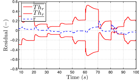
(a) Low Load, \Delta\eta_t = -10\% , \Delta p_{exh} = 0\text{mbar}
