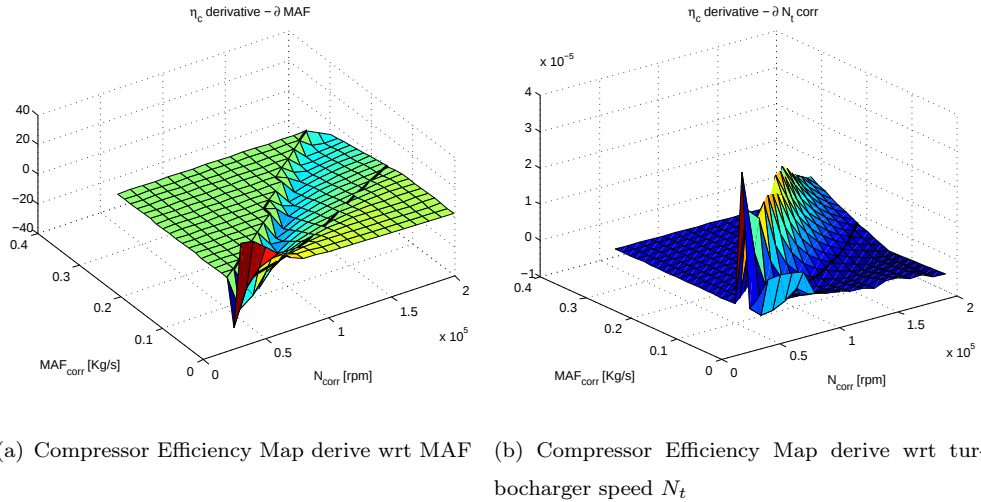
Figure C.1: Compressor Maps
