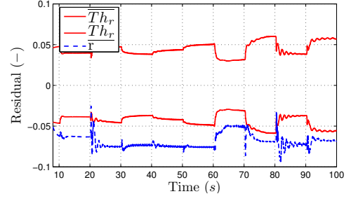
(b) High Load, \Delta\eta_t = -10\% , \Delta p_{exh} = 0\text{mbar}
