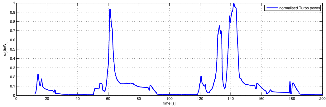
(a) \alpha_t(t)\phi_{W_t}(t)
