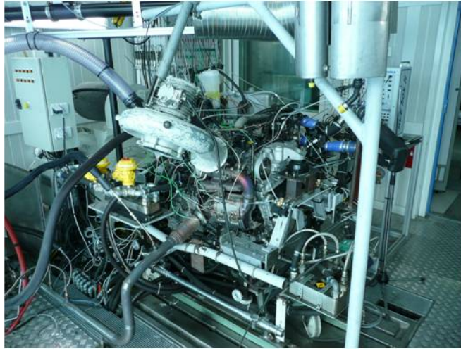
Figure A.2: IFP Test bench: Renault G9T Diesel engine (IFP courtesy)
