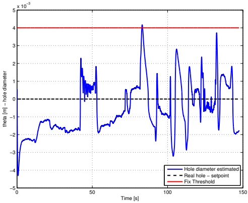
(e) Estimation without leak @2500 rpm
