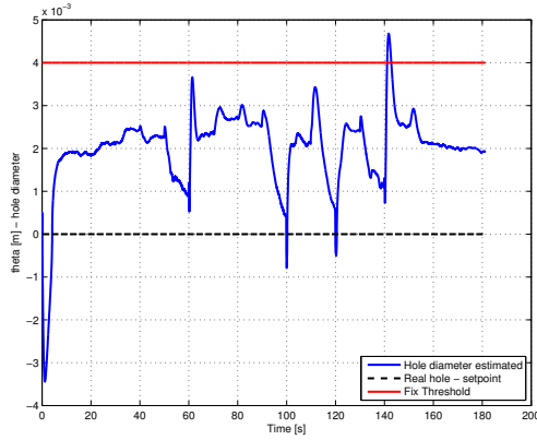
(a) Estimation without leak @1500 rpm
