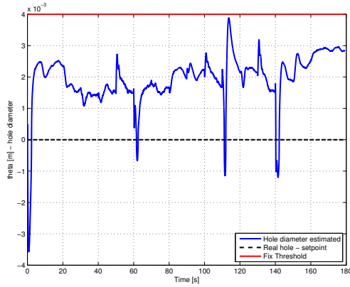
(c) Estimation without leak @2000 rpm
