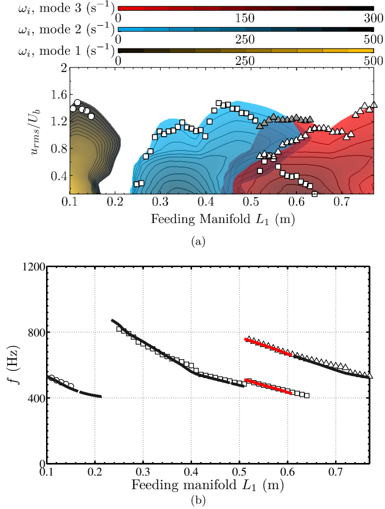
Figure B.8: Theoretical and measured amplitudes (a) and frequencies (b) of unstable modes at limit cycle. Calculations are done with model B by discarding the ring cavity between the two tubes. Experiments are represented by symbols. Open circle symbols ( \circ ) are linked to the first mode while the second mode appears as open square symbols ( \square ) and the third mode as open triangle symbols ( \triangle ). Gray triangle symbols depict the sum of the 2 mode amplitudes (see Chapter 9) in the multiple frequency band ( L_1 = 0.52 m to 0.64 m). For the frequency plot (b), the dark bold lines represent predictions for \omega_i = 0 s^{-1} whereas the red ones correspond to the frequencies of the two modes limit cycles.
