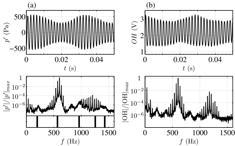
Figure 8.3: Pressure signal recorded by microphone M_2 and OH^* light emission for L_1 = 0.40 m and flame tube L_2 = 0.10 m. Corresponding spectral densities are shown below. The window under the pressure spectrum shows the acoustic eigenmodes positions as vertical solid lines (calculated by assuming that unsteady combustion is absent).
