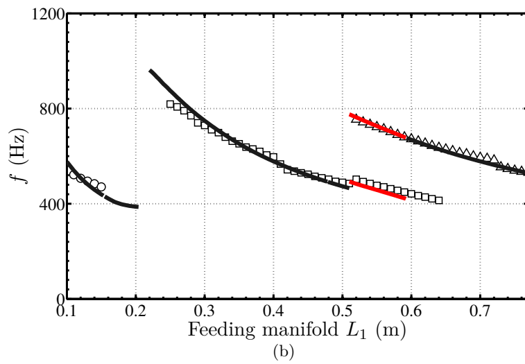
Figure B.2: Theoretical and measured frequencies at limit cycle. Open circle symbols ( \circ ) are linked to the first mode while the second mode appears as open square symbols ( \square ) and the third mode as open triangle symbols ( \triangle ). Dark bold lines represent predictions at \omega_i = 0 \text{ s}^{-1} . The red lines correspond to the dual mode frequencies limit cycle examined in Chapter 9. (a) corresponds to calculations with model B while (b) shows results by considering model A.
