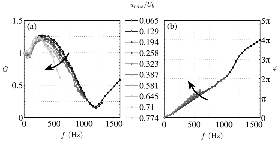
Figure 5.5: FDF measurements for the whole range of amplitudes and frequencies. The perforated plate thickness is set to l = 15 mm with a small flame tube L_2 = 0.10 m. A gray scale shows the increasing level of fluctuations. (a) shows the gain G , while (b) corresponds to the phase \varphi . The decrease of the gain as a function of frequency is more spread compared to data obtained for the thinner perforated plate, while the phase slope is smaller and its amplitude sensitivity less visible.
