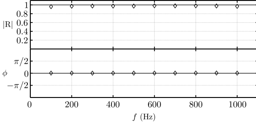
Figure 3.2: Reflection coefficient of the closed end tube measured with the impedance tube device. \diamond symbols indicate measurements, whereas bold lines correspond to the theoretical expected values. One can see that the modulus |R| nearly matches the theory with |R| = 1 while the phase is perfectly equal to 0.
