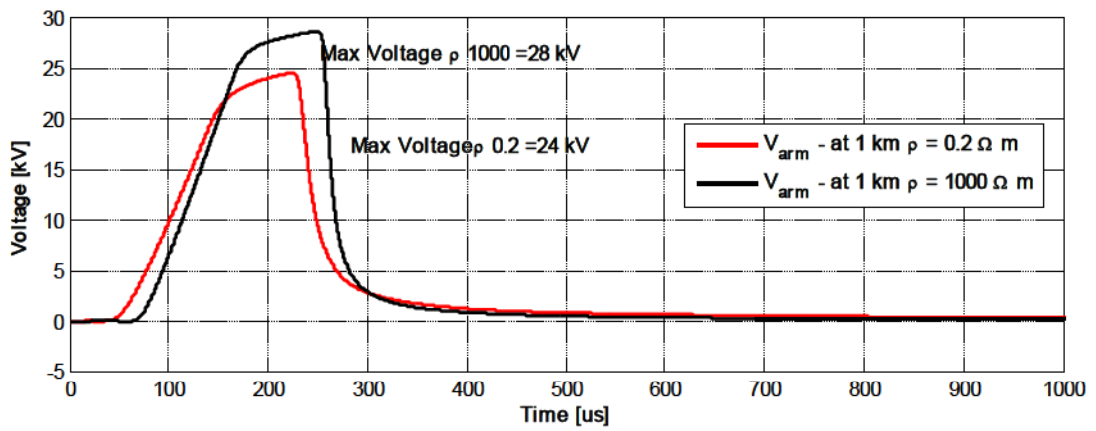
Fig. 53 – Voltage on the armour of the cable using grounding, comparing soil of resistivity 0.2 and 1000 Ω m
