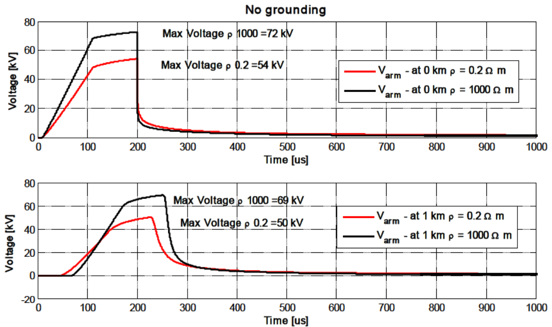
Fig. 52 – Voltage on the armour of the cable without grounding used, comparing soil of resistivity 0.2 and 1000 \Omega m
