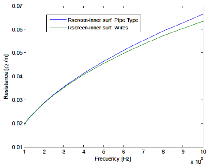
Fig. 58 - Resistance of the inner surface of the pipe - range 10-100 kHz
