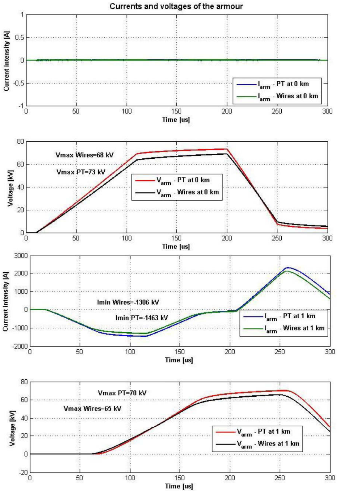
Fig. 50 – Armour currents and voltages at cable entrance and exit – the source is a current ramp between Core A and the ground, no grounding
