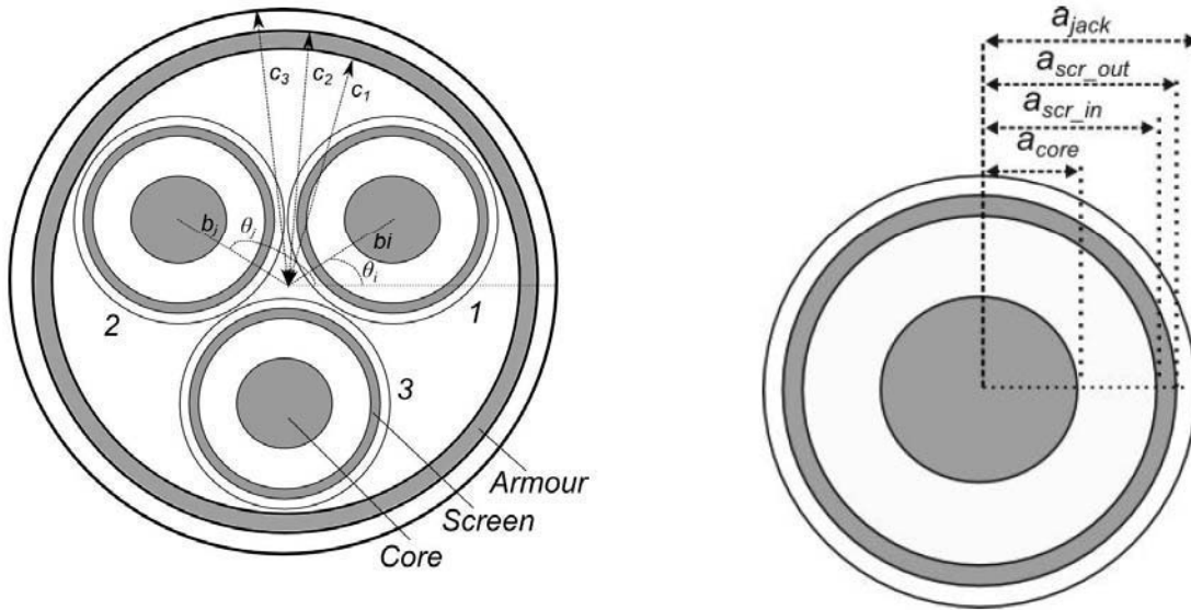
Fig. 43 – Notation of the three-core cable with detail of the inner coaxial cable
