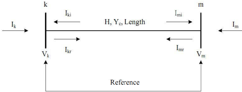
Fig.7 – Single phase line of length L between two nodes (k and m) with impinging current waves, adapted from [18]
