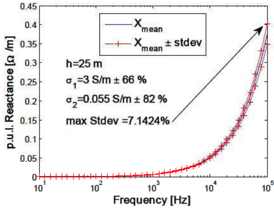
Fig. 40 – Mean resistance and reactance of the sea return impedance, when depth of cable is fixed and conductivities are random variables
