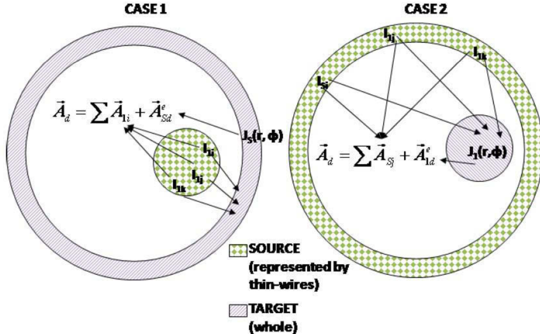
Fig.23 – Two cases (step) used for the calculation of current density distribution in the conductors
