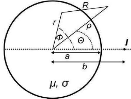
Fig.14 – Transversal section of a circular conductor with a current filament parallel to it
