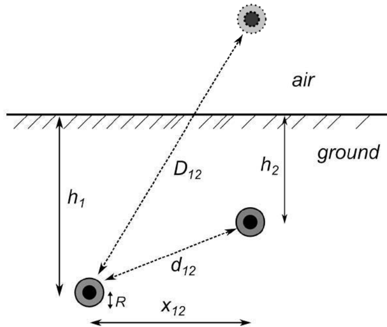
Fig.36 – Configuration used by Pollaczek for the evaluation of ground return term
