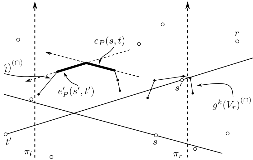
Figure 5.6: The point r is on the right of (s't') and thus on the right of (st) . Hence both edges e_P(s, t) and e_{P'}(s', t') are to remove from g^k(V_l)^{(n)} .
