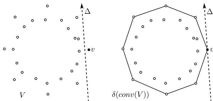
Figure 2.3: The point v (black) can be separated from V \setminus v (white points) by an oriented straight line \Delta , such that v \in \overset{\circ}{\Delta}^- . If \Delta' is parallel to \Delta passing through v , oriented as \Delta , \text{conv}(V) \subset \overset{\circ}{\Delta}'^+ .
