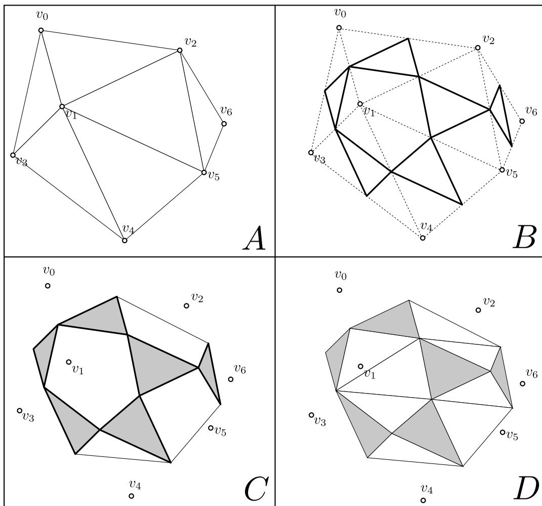
Figure 2.20: Illustration of the order-2 Delaunay triangulation construction: For each order-1 Delaunay triangle we build its corresponding order-2 Delaunay domain triangle (A and B). We later compute the constrained Delaunay triangulation of the 2-set polygon without the domain triangles and we get the order-2 Delaunay triangulation (C and D).
