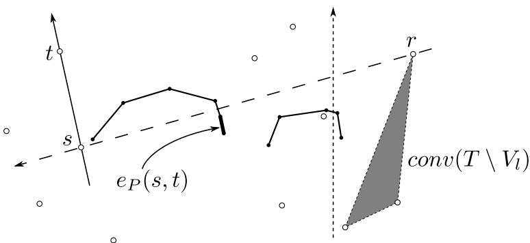
Figure 5.11: Illustration of the proof of Proposition 5.14 (ii).
