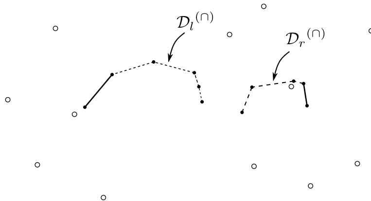
Figure 5.7: The polygonal line \mathcal{D}_l^{(n)} to remove from g^k(V_l)^{(n)} and the polygonal line \mathcal{D}_r^{(n)} to remove from g^k(V_r)^{(n)} .
