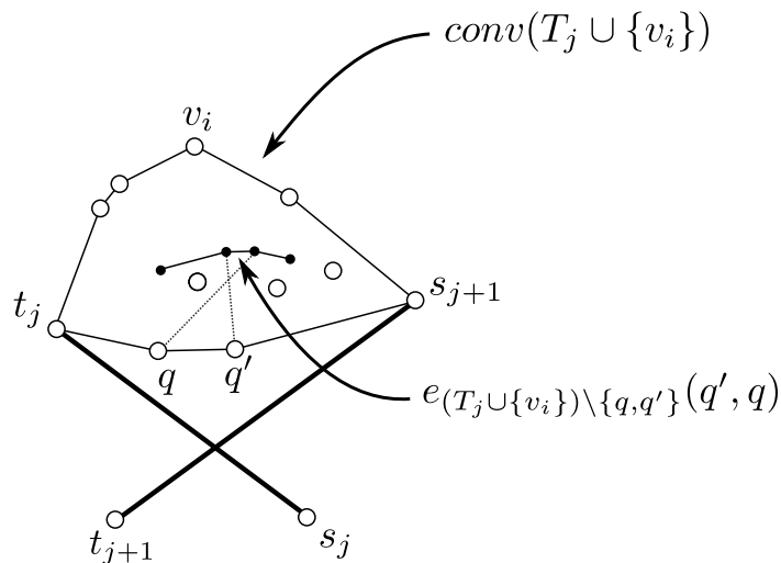
Figure 4.7: Building e_{(T_j \cup \{v_i\}) \setminus \{q, q'\}}(q', q)
