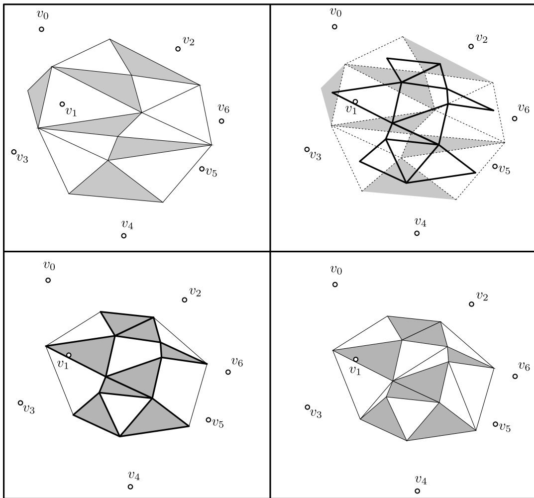
Figure 2.25: An order-3 triangulation obtained from an order-2 triangulation by algorithm build_order_k_triangulation .
