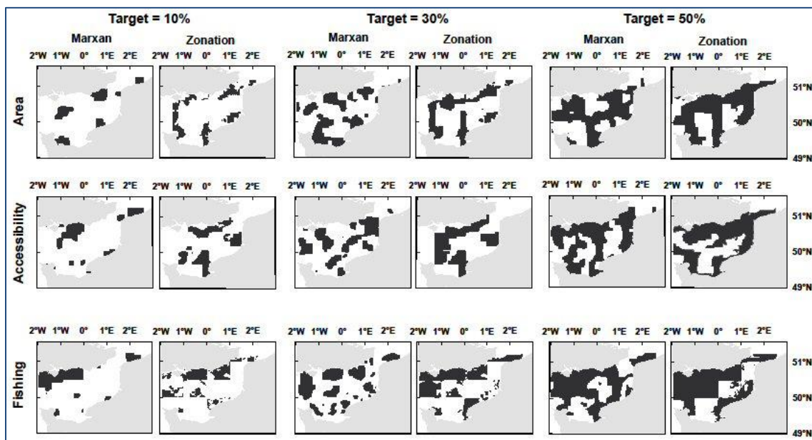
Figure 27: Priority-area maps identified using Marxan and Zonation based on the three different targets and cost metrics.
