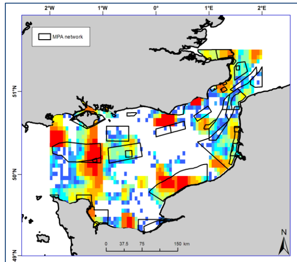
Figure 38: Selection frequency produced with the case 2 cost equation. The MPA network of the EEC is overlaid.
