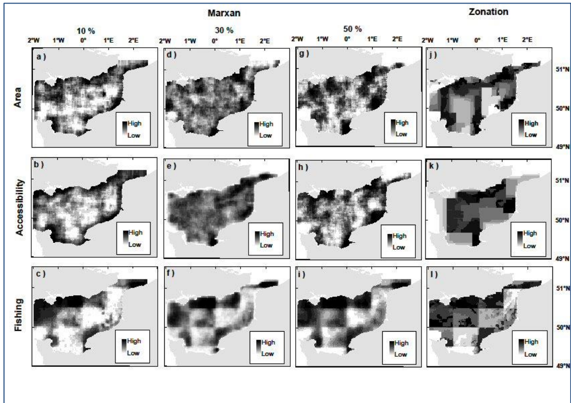
Figure 26: Conservation-value maps for Marxan (a–i) and Zonation (j–l) based on the three different targets and cost metrics. The conservation value for Marxan is based on selection frequency and for Zonation is based on the hierarchical solution output. There are only three maps for Zonation because the hierarchical solution output is a nested output and does not change when using different targets.
