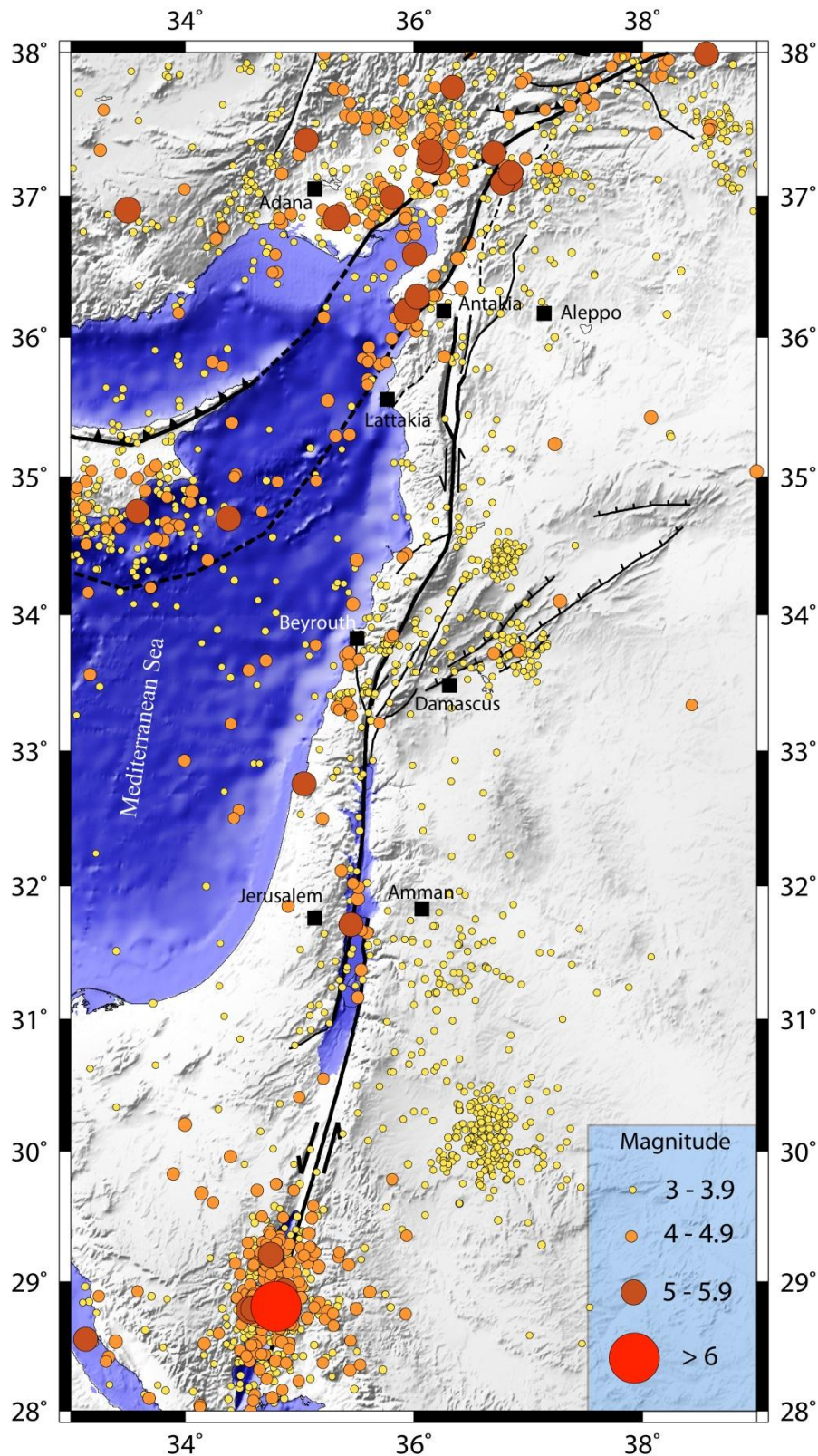
Figure I.4: Instrumental seismicity of the Dead Sea fault between 1964 and 2011, M > 3 . Data are from: IRIS (Incorporated Research Institutions for Seismology, http://www.iris.edu/hq/ ), ISC (The International Seismological Center, http://www.isc.ac.uk/ ) and NEIC (The National Earthquake Information Center, http://earthquake.usgs.gov/regional/neic/ ). Mapped faults are from Meghraoui et al., (2011) and Ferry et al., (2007).
