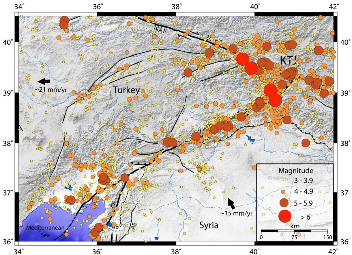
Figure II.3: Instrumental seismicity of the East Anatolian fault between 1964 and 2011, M > 3 . Data are from: IRIS (Incorporated Research Institutions for Seismology, http://www.iris.edu/hq/ ), ISC (The International Seismological Center, http://www.isc.ac.uk/ ) and NEIC (The National Earthquake Information Center, http://earthquake.usgs.gov/regional/neic/ ). Mapped faults from Meghraoui et al., (2011) and Saroglu et al., (1992). KTJ: Karkioiva Triple Junction.
