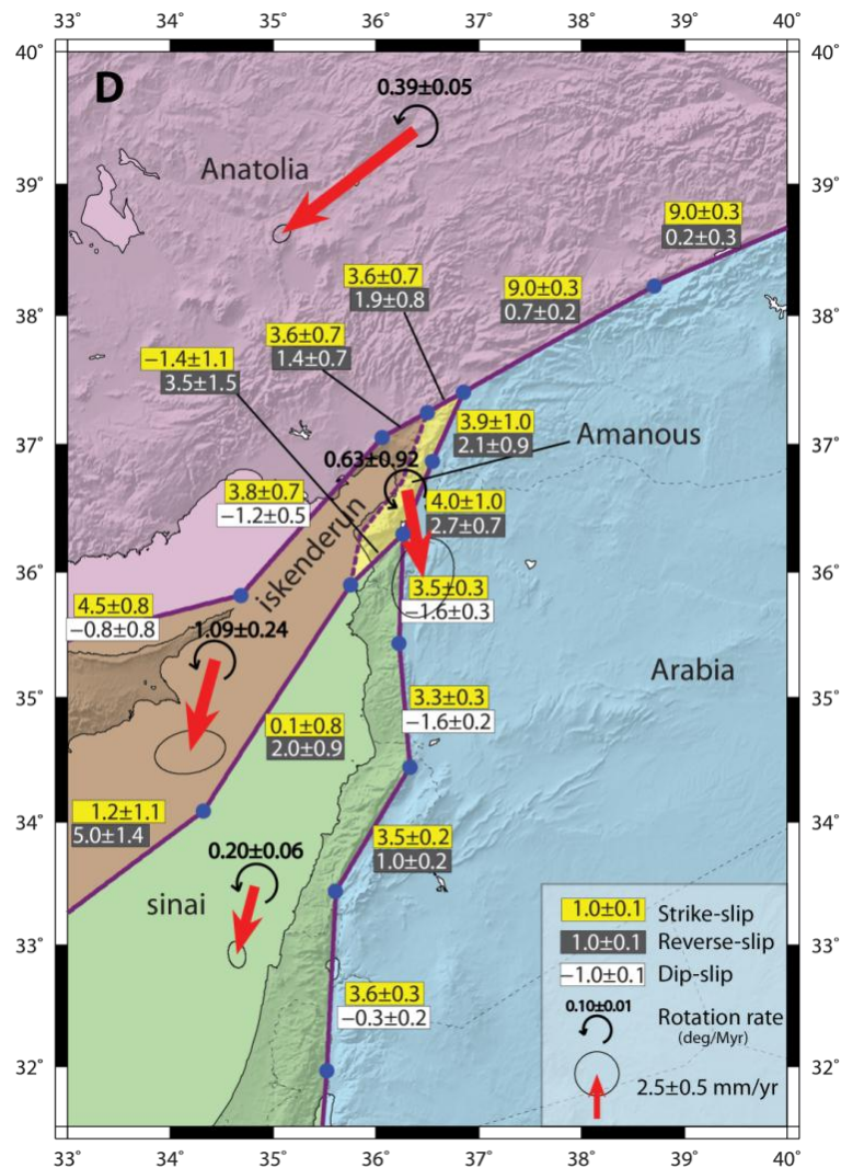
Figure V.3: Illustration of different blocks and relative slip rates on faults in block model D. Red arrows represent GPS-derived block velocity relative to Arabia, and black curve arrows and numbers show the directions and the values of blocks' angular velocities relative to Arabia respectively.
