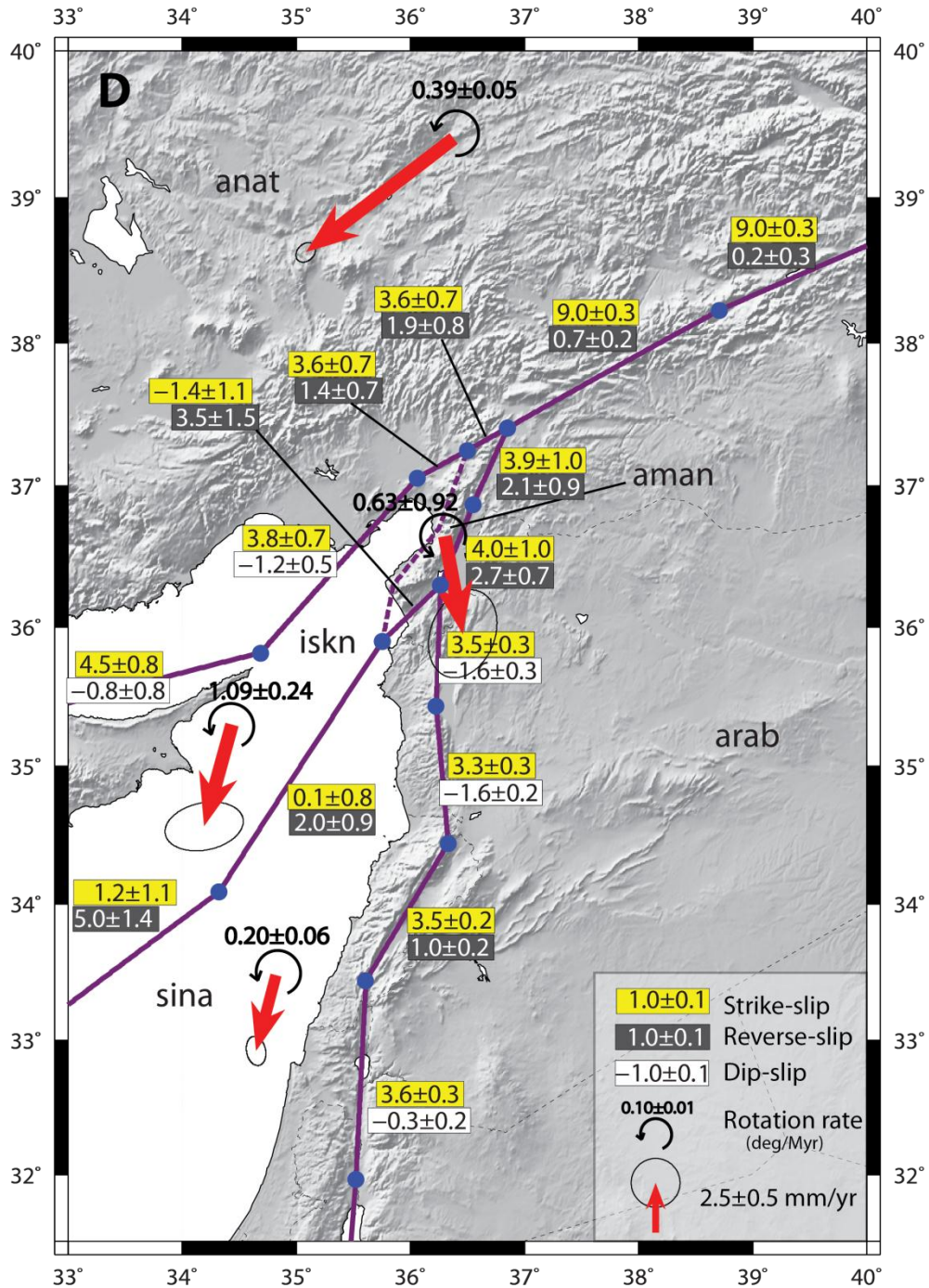
Figure IV.13: Relative slip rates on fault of block model D. Red arrows represent GPS-derived block velocity relative to Arabia, black curve arrows and numbers show the directions and the values of blocks angular velocities relative to Arabia respectively.
