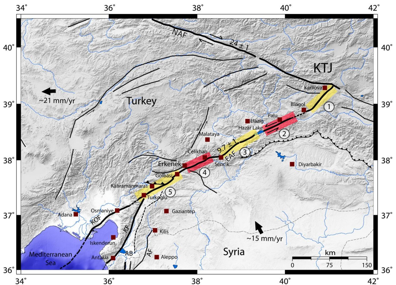
Figure II.1: The East Anatolian fault segments, fault mapping and slip rates from (Westaway, 2003; Meghraoui et al. , 2011). Abbreviations for some key tectonic features: AF: Afrin fault, AB: Amik basin, KF: Karasu fault, KOF: Karatas-Osmaniye fault, EAF: East Anatolian fault. Thick black arrows show the plates convergence Directions. Plate movement rates are from McClusky et al. , (2003); Reilinger et al. , (2006).
