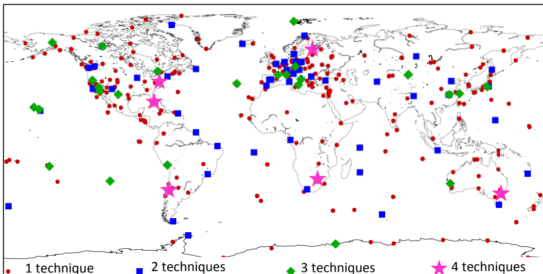
Figure III.3: the ITRF2005 sites with the number of co-located techniques for each site (Altamimi et al. , 2007).
