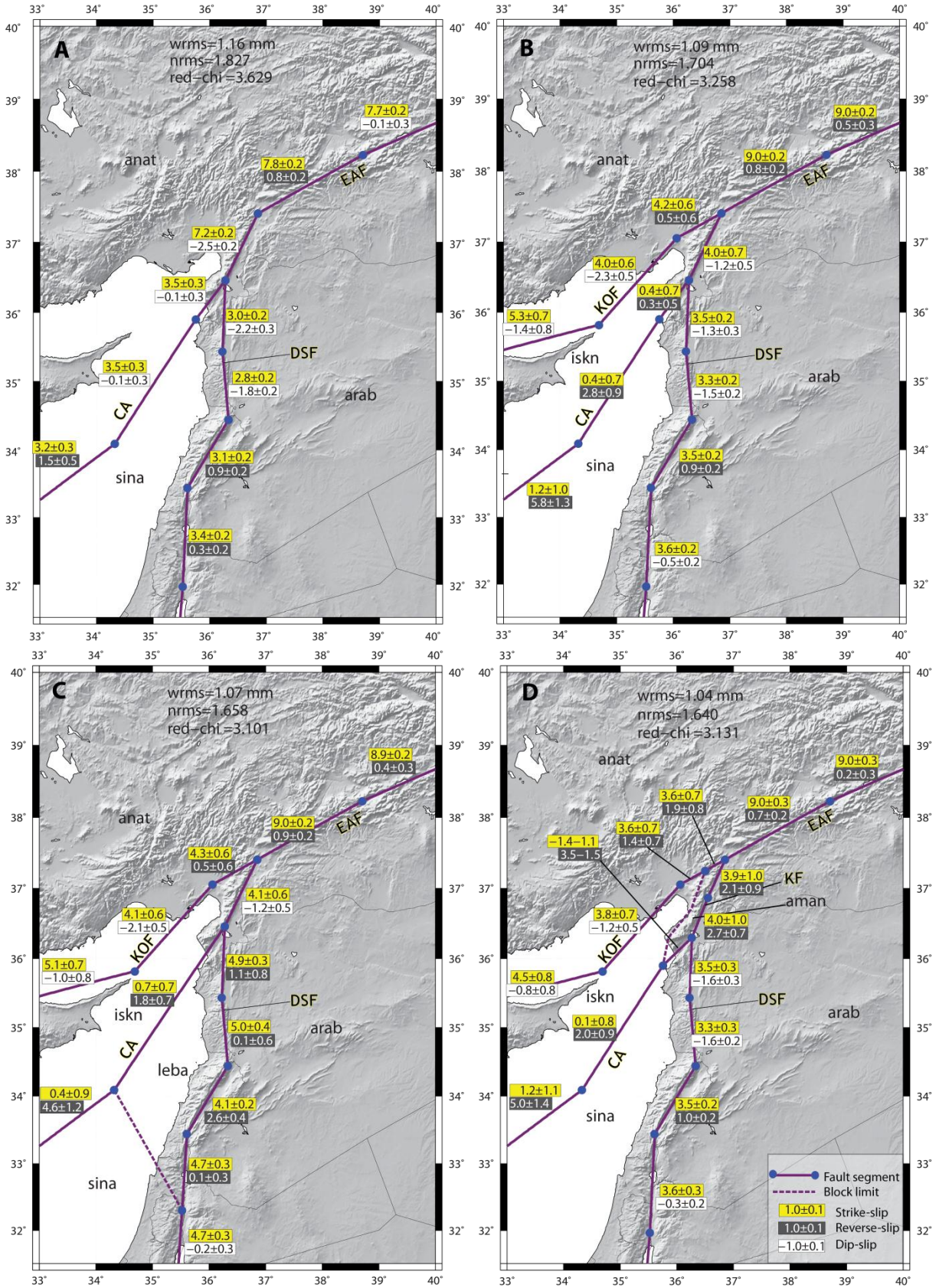
Figure IV.12: Fault slips rates predicted by the four models with different plate configurations. Weighted and normal root mean square and reduced chi square are presented to illustrate model fit. Numbers encountered in yellow rectangles are left-lateral strike-slip rate (mm/yr).
