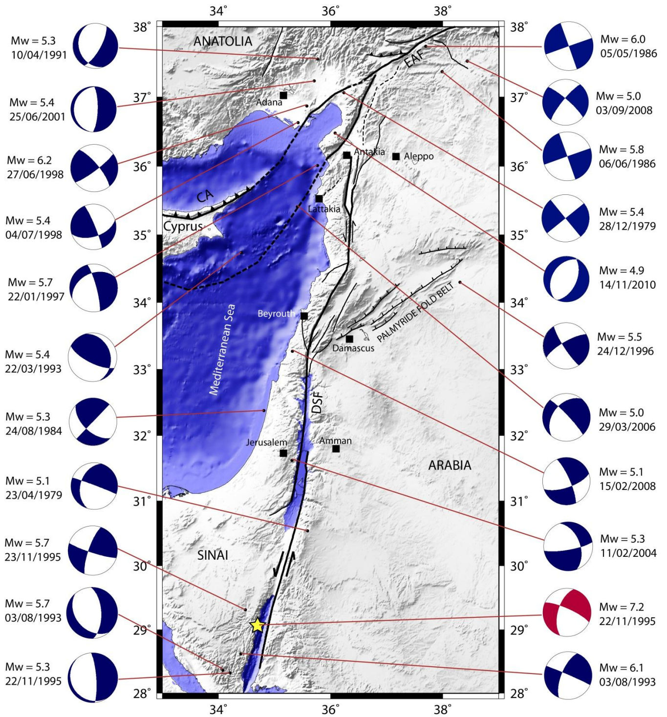
Figure I.5: Focal mechanism of earthquakes between 1976 and 2011 along the Dead Sea Fault, of magnitude greater than 4.5. Data are from catalogues Harvard CMT. Mapped faults are from Meghraoui et al., (2011) and Ferry et al., (2007).
