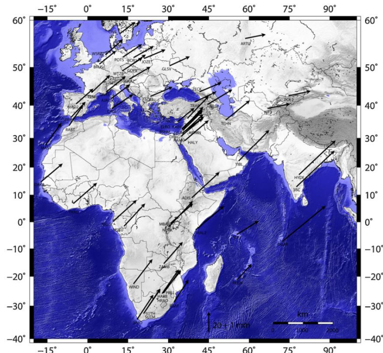
Fig. 4. GPS velocity field of the 50 IGS permanent stations used in this study to constrain our observations to the global GPS network and their 95% confidence ellipses shown in the ITRF05 reference. Data are from January 1999 to December 2010.
