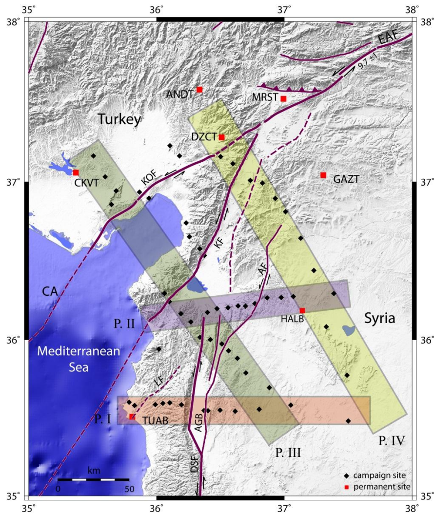
Figure III.4: Map illustrate the campaign GPS sites (black diamonds) in North-West Syria and South-East Turkey and a part of the regional CGPS sites (red squares) used in this study. The colored rectangles refer to the 4 GPS profiles mentioned previously. Abbreviations for some
