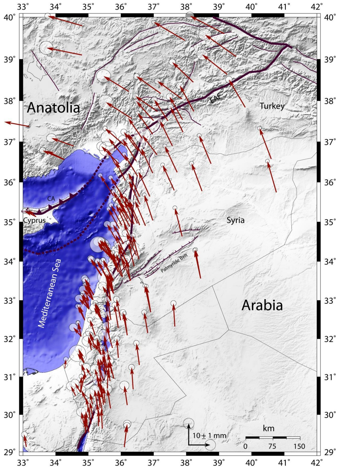
Figure 1.6: GPS Horizontal velocity field and the 95% confidence ellipses obtained by previous campaigns in the Eastern Mediterranean region with respect to the Eurasia-fixe reference frame. GPS data are from Reilinger et al., 2006, Gomez et al., 2007 and Le Béon et al., 2008. Mapped faults are from Meghraoui et al., 2011. Also shown in the map are the three major faults in the region, EAF: East Anatolian fault, DSF: Dead Sea fault, CA: Cyprus arc.
