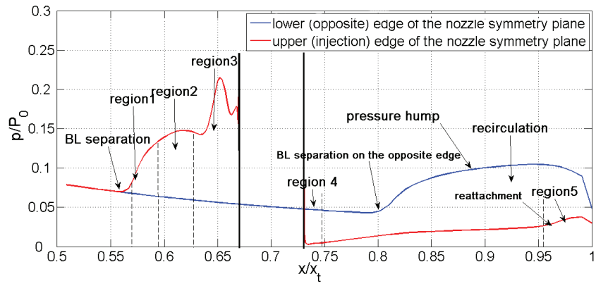
(a) Wall-pressure profiles
