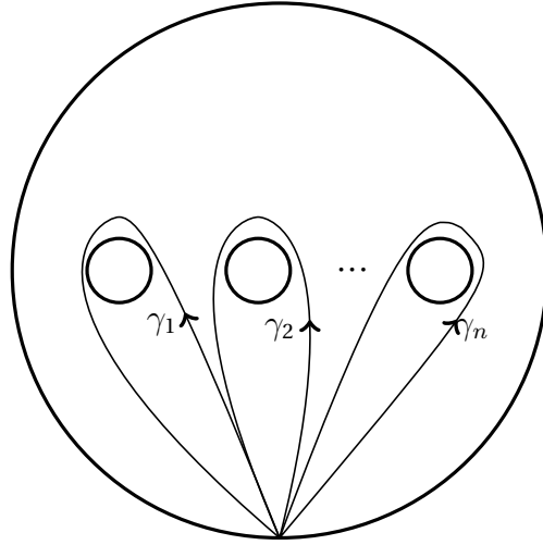
FIGURE 1 – \pi_1(D_n)
