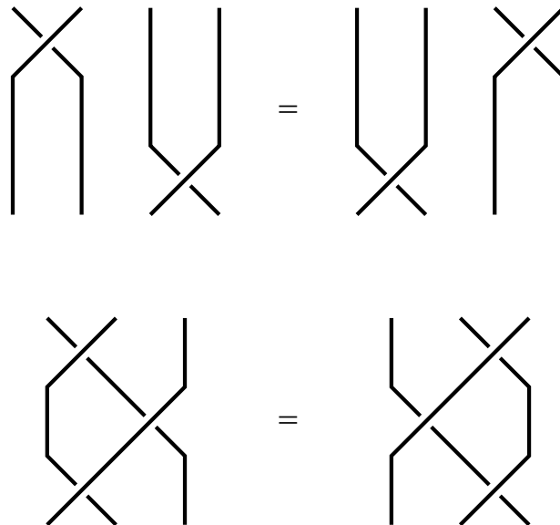
FIGURE 2 – Relations d'Artin
