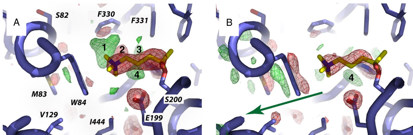
Fig. 3. OTMA in the CAS of TcAChE at 100 K ( A ) and 150 K ( B ). Protein residues are shown in blue, and the OTMA molecule is shown in yellow. The Fourier difference maps (contour level 4\sigma ) computed for data sets IV – I at 100 K ( A ) and for data sets III – I at 150 K ( B ), are shown superimposed on the model. Positive and negative peaks are shown in green and red, respectively. Peaks 1–4 are referred to in the text. The arrow in B indicates a putative backdoor exit of PsCh that is also indicated by a green arrow in Fig. 2. The orientation in Fig. 3 is the same as in Fig. S1 but slightly zoomed out. A version for the colorblind is given in Fig. S2.
