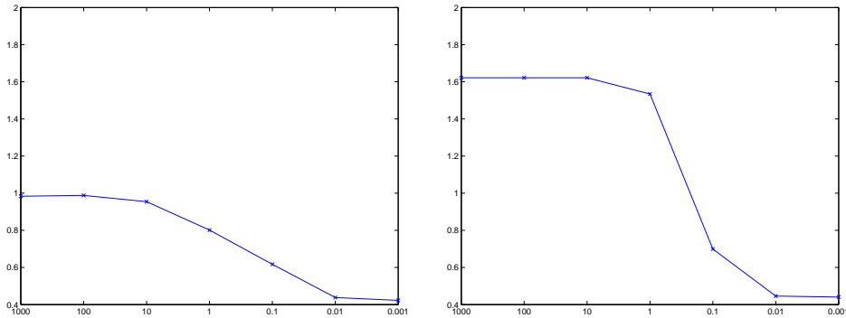
Figure 6.10: L^1 error (6.30) on the distribution of S_0^\epsilon for m = 20 . Left: initial condition Y_0 = (0, 0) . Right: initial condition Y_0 = (10, 1) .
