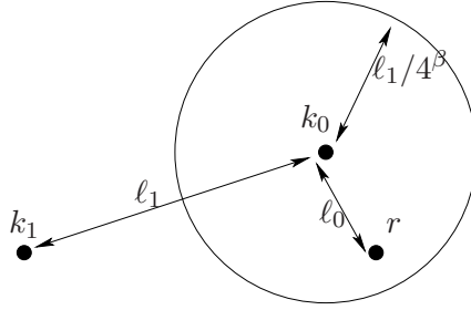
Figure 3.4: A configuration of r , k_0 and k_1 where \ell_0 \leq \ell_1/4^\beta used in the proof of Lemma 3.7.2.
