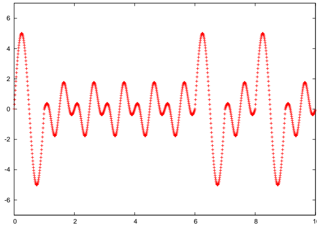
Figure 4.4: A realization of the potential V .
