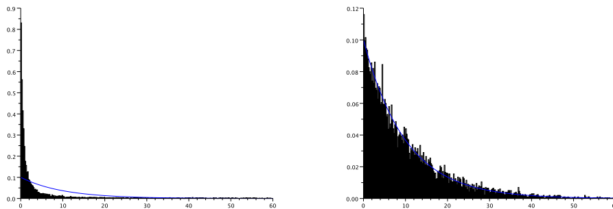
Figure 6.4: Distribution of S_0^\varepsilon , the first exit time from a macro-state ( m = 20 ). Left: large \varepsilon = 1 . Right: small \varepsilon = 10^{-3} .
