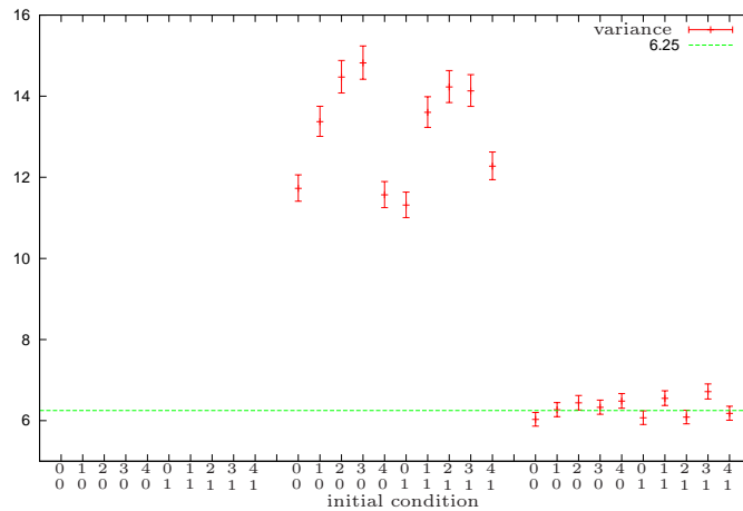
Figure 6.7: Empirical variance of S_0^\epsilon for different initial conditions and different values of \epsilon , with the same convention as on Fig. 6.6 (results for \epsilon = 10^3 do not fit in the chosen y-range).
