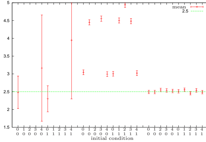
Figure 6.6: Empirical expectation of S_0^\epsilon for different initial conditions and for \epsilon = 10^3 (left), \epsilon = 1 (center) and \epsilon = 10^{-3} (right). Initial conditions are shown on the x-axis in the format \begin{pmatrix} X_0 \\ Z_0 \end{pmatrix} \in \begin{pmatrix} M \\ \{0, 1\} \end{pmatrix} , with M = \{0, 1, 2, 3, 4\} .
