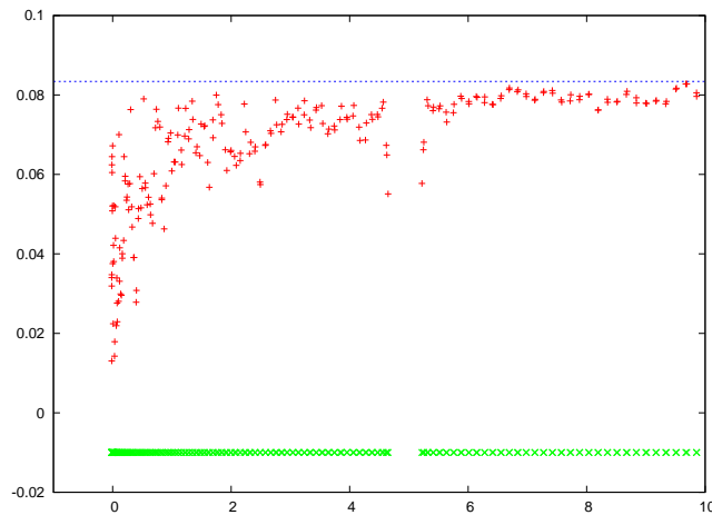
Figure 1.10: The spectrum of the mean-field Hamiltonian H(\omega) is represented in green. The y -axis represents the values of the variance v that quantify the "spreading" of the eigenfunctions. Each red dot represents the variance v of the eigenfunction corresponding to the eigenvalue in the same vertical line. The blue line indicates the maximal value of v .
